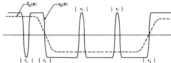
FIG. 3. Visualization of the renormalization process: We replace S_2(\beta) by a long-term average including the effect of all spin-flip pairs closer together than \tau_1 .
