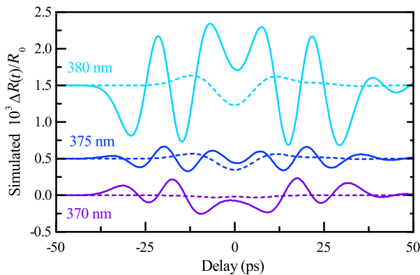
FIG. 4. Simulation for the relative reflectivity change \Delta R/R_0 due to the photoelastic effect in the GaN bulk layer (solid lines) and the interface displacement (dashed lines) for the three studied wavelengths \lambda . The curves are shifted vertically for clarity.
