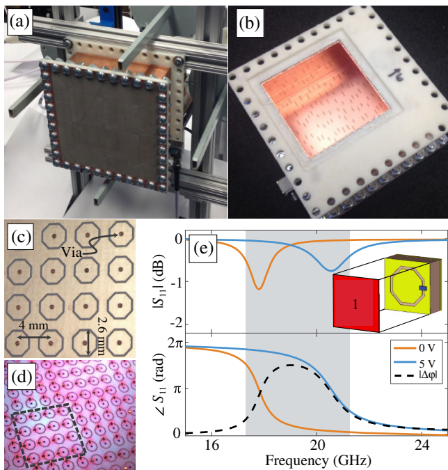
FIG. 2. (a) The cavity implemented in the imaging configuration, including four open-ended waveguide receivers. A network analyzer and mechanical switch are situated behind the aperture to take the measurements from the different receivers. (b) The interior of the cavity when the impedance surface is removed. (c) An enlargement of the particular mushroom structure and (d) a highlighted pixel on the varactor-populated impedance surface. (e) The full-wave simulation domain and results for a mushroom unit cell.
