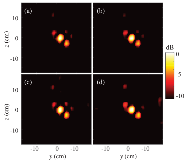
FIG. 10. Single-frequency images of a subresolution scatterer (a centered 1.5-cm-diameter sphere) with different quantities of measurements. Quality remains the same between (a) 200 and (b) 150 but slowly degrades for (c) 100 and (d) 50 measurements. Note that the angular skew in the PSF is induced by the asymmetric alignment of the receiving antennas.
