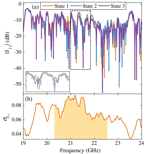
FIG. 3. (a) Return loss of the perforated cavity with a dense frequency sampling. Three example states are shown as well as an enlargement (contained by the dashed box). (b) The standard deviation of the return loss is also plotted for a set of 100 measurements and the bandwidth used for imaging is highlighted.
