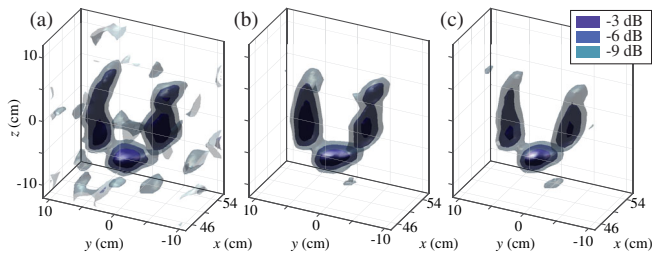
FIG. 7. (a) Passive-mode reconstruction of the letter U obtained with 201 frequency points. (b) Dynamic reconstruction with approximately the same number of measurements ( N = 208 ) and (c) dynamic result with half as many measurements ( N = 104 ).
