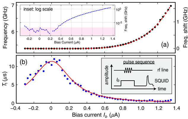
FIG. 2. Frequency shift \delta f_Q and energy relaxation time T_1 versus pulse amplitude I_b . (a) \delta f_Q versus I_b . The data (black dots) are fit (red line) using Eq. (3) to 4th order in I_{bs} , with \alpha = 1.0 \times 10^5 A -1 , and \beta = 1.6 \times 10^{16} A -3 . Inset: frequency shift on log scale. Data in pink region are not well resolved due to the frequency step-size used. (b) T_1 versus I_b . Data (blue dots) are fit (red line) to 1/T_1 = 1/T_1^{(0)} + \kappa(I_b - I_b^*)^2 . T_1^{(0)} = 12 \mu s is the qubit's energy decay time at I_{bs} = 0 ; \kappa = 1.27 \times 10^{18} A -2 /s. Inset: pulse sequence of the experiment.
