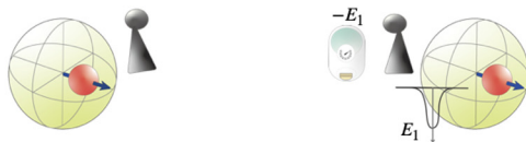
FIG. 1. Quantum gate operations used for quantum energy teleportation. (a) Preparation of the ground state and Alice's X_0 measurement to deposit her energy. She tells Bob via classical communication whether \mu = -1 or \mu = +1 was observed. (b) Bob's conditional operations to receive energy. He selects an operation U_1(+1) or U_1(-1) based on \mu = +1 or -1 , corresponding to the Maxwell demon operation. (c) Equivalent implementation of Bob's operations on a quantum computer.
