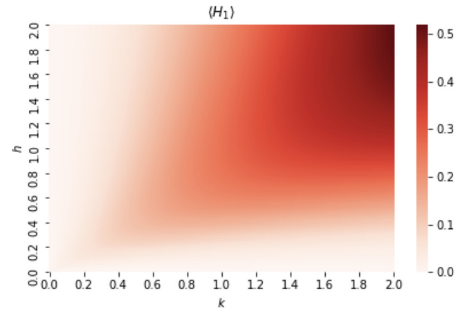
FIG. 3. Heat maps visualizing expectation values \langle V \rangle = \text{Tr}[\rho_{\text{QET}}V] and \langle H_1 \rangle = \text{Tr}[\rho_{\text{QET}}H_1] by (k, h) .
