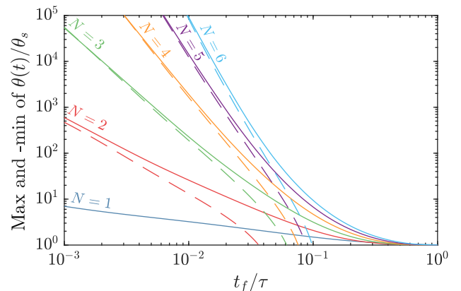
FIG. 12. Maximum (plain line) and opposite of the minimum (dashed line) values of \theta(t) for N = 1 to 6, t_f/\tau = 10^{-3} to 1, and \tilde{x}_0 = 0.95 . Large N and short t_f lead to a huge transient temperature, limiting the magnitude of achievable temperature step \theta_s . No negative values of \theta(t) are observed for N = 1 .
