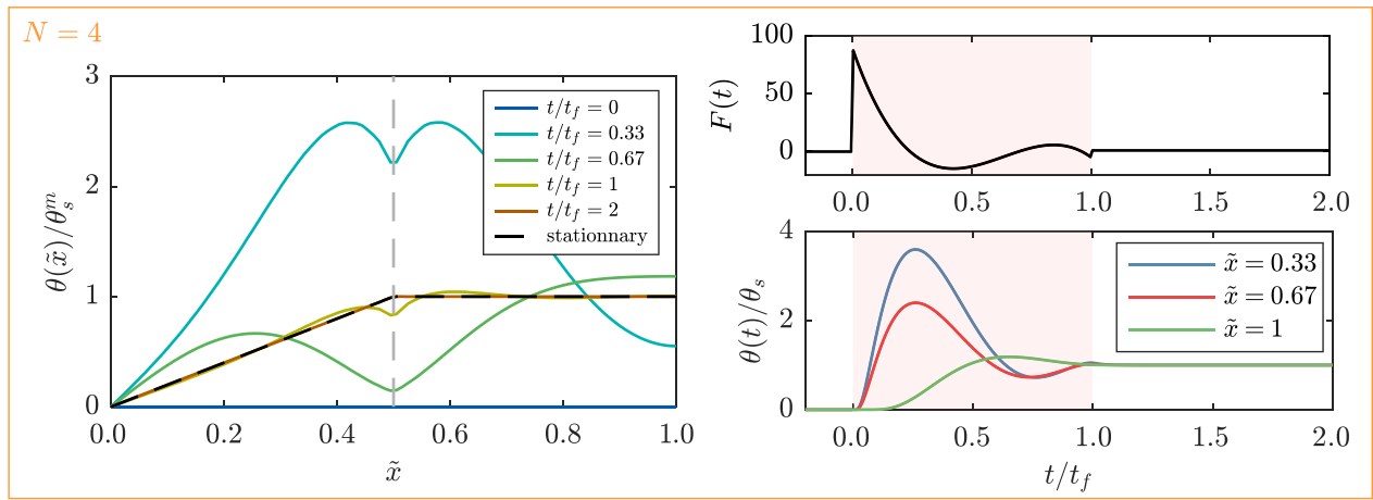
FIG. 10. Numerical simulation of the protocol for the same parameters as in the bottom panel of Fig. 4: N = 4 , t_f = 0.1\tau , but a different value of the heating location, \tilde{x}_0 = 0.5 .
