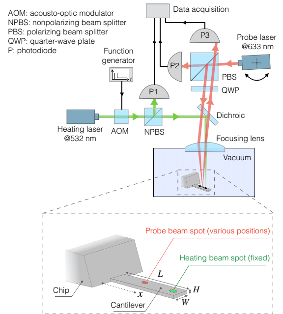
FIG. 2. Sketch of the experimental setup. The heating laser beam (at 532 nm) is fixed and focused at the extremity of a cantilever placed in vacuum. The power of the heating beam is modulated with an acousto-optic modulator. The probe laser beam (at 633 nm) is used to measure the local temperature change by analyzing the cantilever reflectivity variations. By tilting the probe laser, the probe beam spot scans the cantilever length allowing measurement of the temperature variation at different positions x .
