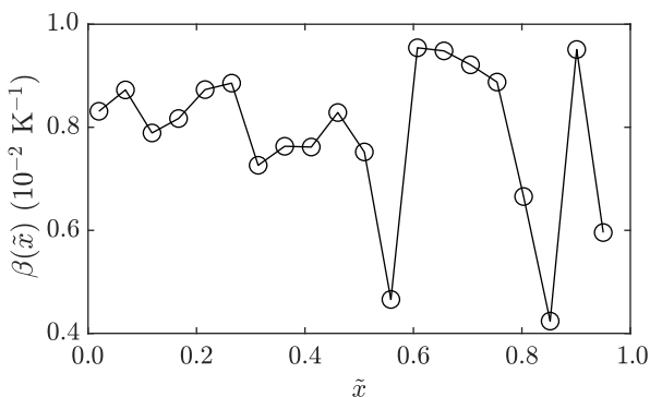
FIG. 11. Calibration of the sensitivity coefficient \beta . This quantity makes it possible to convert the variation of reflectivity into temperature change, \theta(x) = \beta^{-1}(x)\Delta R(x)/R(x) . The relatively large range of dispersion for the sensitivity \beta is mainly due to variations of the thickness along the cantilever length.
