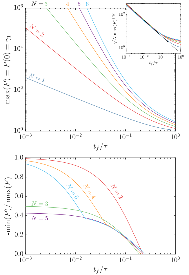
FIG. 9. (Top) Maximum value of F(t) , corresponding to F(0) = \gamma_1 , for N = 1 to 6 and t_f/\tau = 10^{-3} to 1. Large N and short t_f lead to a huge range of power needed during the transient. A scaling \max(F) \sim [0.45\tau/(t_f \sqrt{N})]^N is observed, as illustrated in the inset (dashed line is 0.45\tau/t_f ). (Bottom) Minimum value of F(t) , normalized by its maximum value, for N > 1 [for N = 1 , F(t) > 0 at all times, thus no cooling is necessary]. The cooling power is always smaller in absolute value than the heating one.
