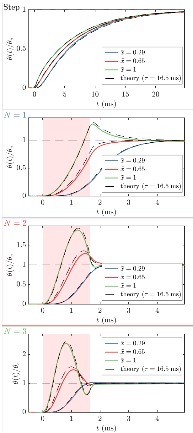
FIG. 8. Transient temperature profiles measured when applying a step function and the accelerating protocol ( N = 1 up to N = 3 ) for a maximum temperature elevation \theta_s^m = 1 K. The small deviation from theory is attributed to the thermal conductivity dependence of silicon with temperature: as the initial profile corresponds to a maximum temperature rise of 50 K, \lambda is up to 16% smaller near the cantilever's free end.
