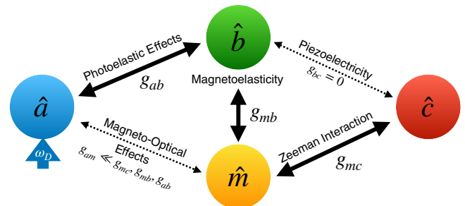
FIG. 1. Sketch of a two-stage interconversion protocol between optical and microwave photons respectively represented by \hat{a} and \hat{c} . The two intermediary states are \hat{b} , phonons, and \hat{m} , magnons, both with frequencies in the microwave range. The thick lines denote the dominant interaction scheme.
