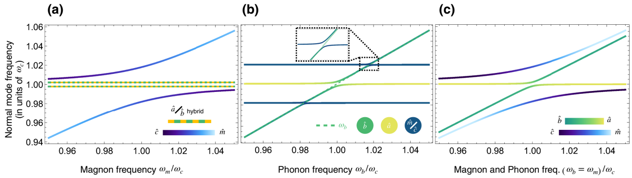
FIG. 4. Plot of the hybridization ratio of the four waveforms as a function of their detuning. The avoided crossing region is shown in the rotating frame of the driven optical cavity, stemming from the interaction chain shown in Fig. 2, as a function of (a) the magnon frequency \omega_m , (b) the phonon frequency \omega_b , and (c) both set equal and simultaneously tuned. The color code corresponds to the weights of the different bare modes, and shows how the hybrid mode is formed as a combination of the bare modes. We normalize all frequencies by the fixed microwave frequency and set \omega_c = -\Delta_a . We set the optical pump power P = 10^{-4} W, corresponding to a photon-phonon cooperativity C_{ab} = 1124 ; and the magnon-phonon cooperativity C_{mb} = 4 \times 10^5 and magnon-microwave cooperativity C_{mc} = 1258 , corresponding to the estimates presented in Table I.
