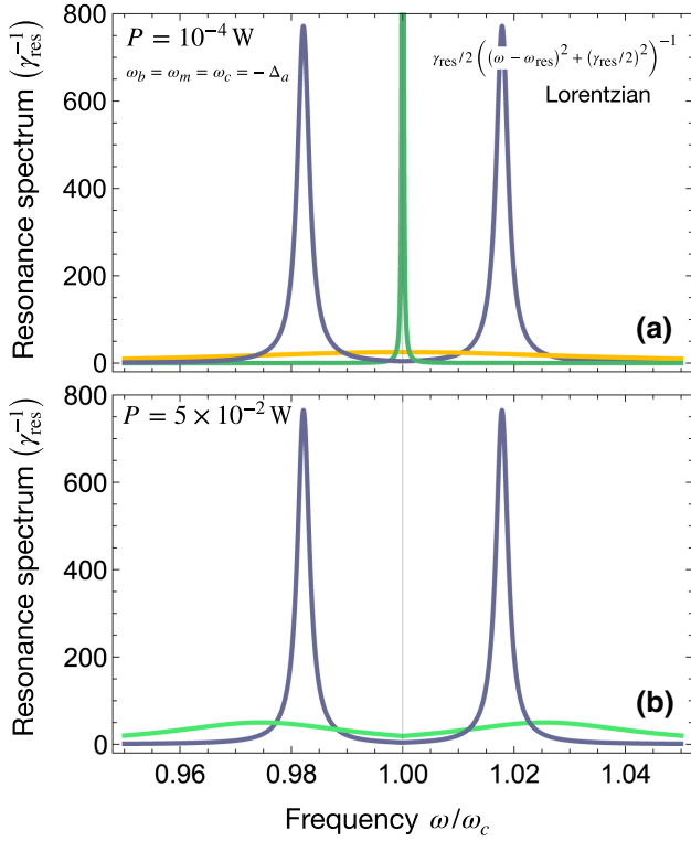
FIG. 5. Frequency spectrum of the resonances of the coupled system defined by Eqs. (9). The spectrum is obtained when all modes are on resonance, including the optical detuning. The blue peaks correspond to the magnon-microwave hybrid modes. We assume full mode degeneracy ( \omega = \omega_m = \omega_b = \omega_c = -\Delta_a ) and, based on the estimates of Table I, we fix cooperativities at C_{mb} = 4 \times 10^5 and C_{mc} = 1258 for magnomechanics and magnon-microwave coupling, respectively. Spectra are depicted for pump powers of (a) 10^{-4} ( C_{ab} = 1124 ) and (b) 5 \times 10^{-2} W ( C_{ab} = 562\,353 ). In (a) the system is in the weak optomechanical coupling regime, and hence no resolved shift of the phonon (green) and photon (yellow) modes. In (b) the system exhibits strong optomechanical coupling and therefore a normal mode splitting (light green) becomes evident.
