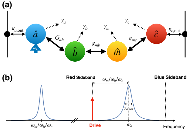
FIG. 2. (a) Schematic and notation of the quadripartite coherent interconversion protocol showing the interdependence of the four different waveforms. The chain arises from selecting the dominant coupling mechanisms in Fig. 1. Here, \kappa_{a/c,\text{out}} denotes coupling to the optical or microwave port and \gamma_{a/b/m/c} are the intrinsic linewidths of each waveform. We consider an optical pump at frequency \omega_D and therefore the optomechanical coupling is enhanced and denoted by G_{ab} . (b) Pumping scheme for driving of the red sideband of the optical cavity. Here \omega_a, \omega_b, \omega_m and \omega_c correspond to the optical photon, phonon, magnon, and microwave photon modes, respectively.
