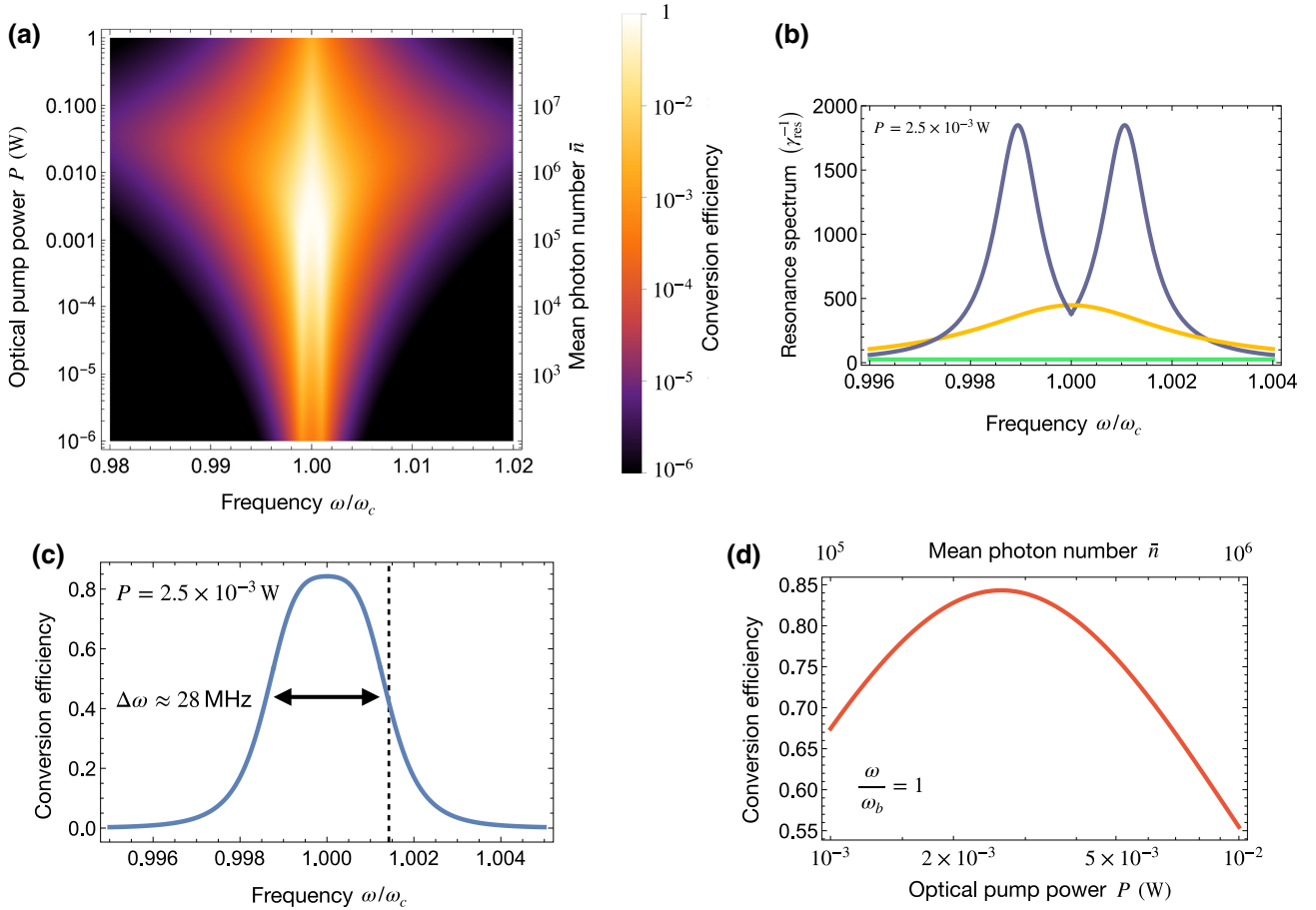
FIG. 9. (a) Conversion efficiency as a function of frequency and optical pump power (corresponding mean photon number on the right y axis). The frequency axis is given in units of \omega_c , the microwave frequency, and we have set \omega_b = \omega_m = \omega_c = -\Delta_a . (b) Frequency spectrum of the resonances of the coupled system following Eqs. (9). In this case the blue peaks correspond to the magnon-phonon hybrid modes. Since the system is still in the weak optomechanical coupling regime for the used optical pump power of P = 2.5 \times 10^{-3} W ( C_{ab} = 28\,118 , C_{mc} = 13 ), the phonon (yellow) and photon (green) are not shifted. (c) Conversion efficiency as a function of frequency for the point of highest efficiency at a pump power of about P = 2.5 \times 10^{-3} W. The remarkably large bandwidth at this point is marked with 28 MHz. (d) Conversion efficiency as a function of optical pump power.
