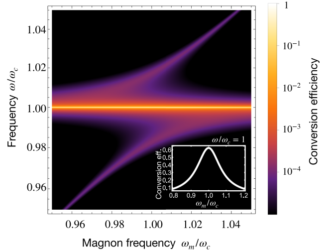
FIG. 6. Conversion efficiency, Eq. (11), as a function of frequency \omega and magnon frequency \omega_m , both in units of the fixed microwave frequency \omega_c . The phonon frequency \omega_b and optical detuning are set to -\omega_c . The white inset shows the conversion efficiency at \omega/\omega_c = 1 as a function of magnon frequency. The optical pump power is set to P = 10^{-4} W, corresponding to the cooperativity C_{ab} = 1124 . Other parameters are fixed according to the estimates in Table I, corresponding to C_{mb} = 4 \times 10^5 and C_{mc} = 1258 .
