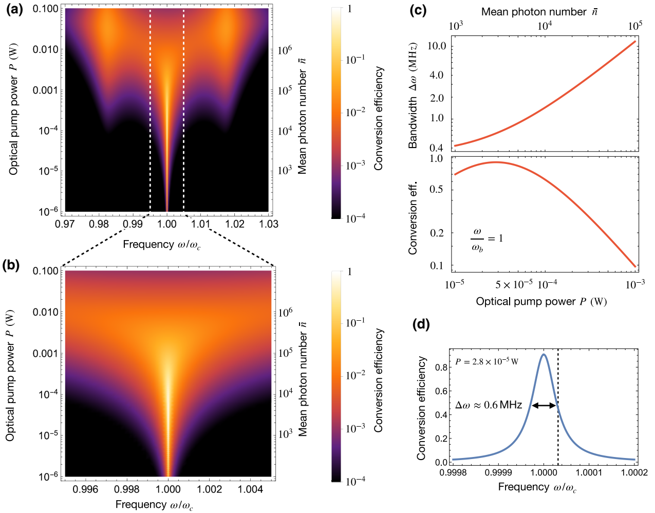
FIG. 7. (a) Conversion efficiency as a function of frequency and optical pump power (corresponding mean photon number on the right y axis). The frequency axis is given in units of the microwave mode frequency \omega_c and the color code for the conversion efficiency is given on a logarithmic scale. We set \omega_b = \omega_m = \omega_c = -\Delta_a . The lower plot (b) is an enlargement of the upper plot. (c) Bandwidth and the respective conversion efficiency as a function of optical pump power. (d) Conversion efficiency as a function of frequency for the point of maximum efficiency at a pump power of 2.8 \times 10^{-5} W, corresponding to a cooperativity C_{ab} = 320 . The bandwidth at this point is marked with 0.6 MHz. Other parameters are in correspondence with the estimates shown in Table I for which C_{mb} = 4 \times 10^5 and C_{mc} = 1258 .
