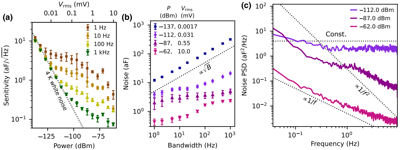
FIG. 3. (a) The measured sensitivity of the capacitance measurement. The dotted line indicates the sensitivity limit due to the amplifier noise ( T_{noise} \approx 4 K). (b) The standard deviation of the gate capacitance measurement versus the vector network analyzer bandwidth. The dotted line indicates the scaling of the noise \propto \sqrt{B} , expected for white noise such as Johnson-Nyquist noise. (c) The capacitance noise power spectrum (PSD) for a measurement bandwidth of 50 Hz.
