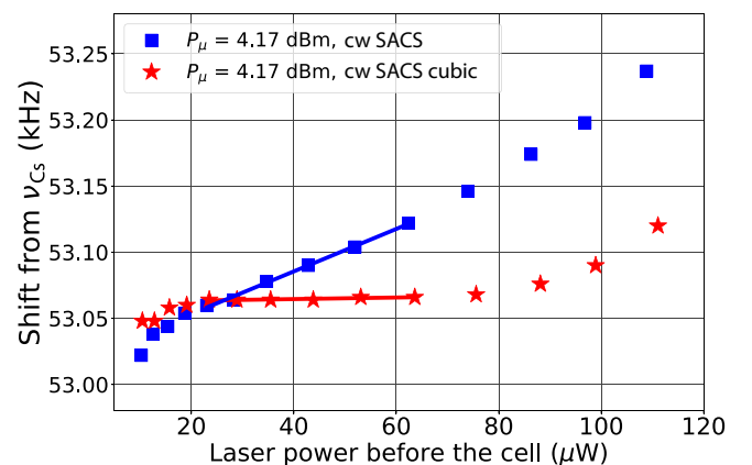
FIG. 6. Clock frequency shift (referenced to \nu_{\text{Cs}} ) versus the laser power at the cell input using cw ACS with two different approximations (squares, linear; stars, cubic) for the light-shift dependence. The microwave power is P_\mu = 4.17 dBm. Error bars are smaller than the data-point symbols. Solid lines indicate a linear fit to the data points, in the 20–63- \mu\text{W} range.
