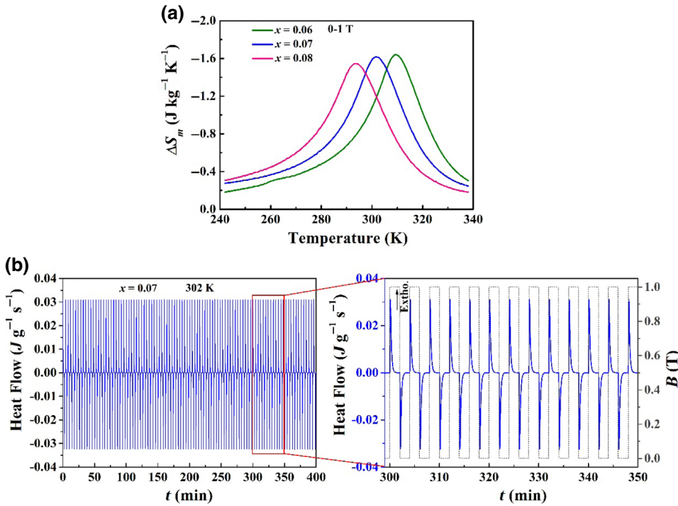
FIG. 6. (a) Temperature dependence of \Delta S_m for a field change of 0–1 T for the MnCo 1-x Cu x Ge ( x = 0.06, 0.07, and 0.08 ) alloys. (b) Heat flow for 100 cyclic magnetic fields of 0–1 T for the sample with x = 0.07 at 302 K.
