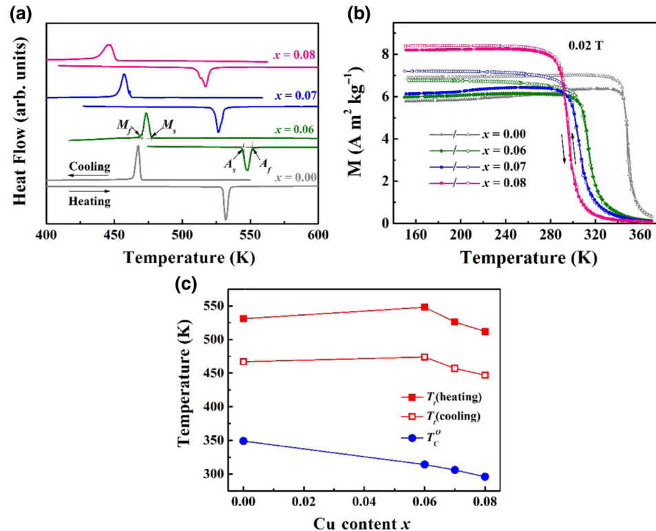
FIG. 3. (a) DSC curves and (b) M-T curves in a field of 0.02 T in heating and cooling processes for MnCo_{1-x}Cu_xGe alloys. (c) Evolution of characteristic temperatures, T_i (heating), T_i (cooling), and T_c^0 , as a function of Cu content.
