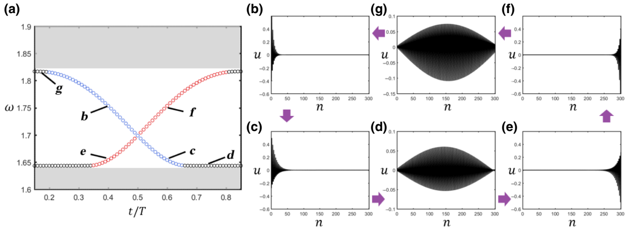
FIG. 5. (a) The edge states within the higher band gap at t=0.4T and t=0.6T are labeled b, e , and c, f ; the bulk states at t=0.75T and t=0.15T are labeled d and g . The corresponding eigenmodes as a function of position along the 1D lattice are plotted in (b)–(g), respectively, where n is the mass index and u the corresponding displacement amplitude. The shaded gray regions indicate the bulk pass bands.
