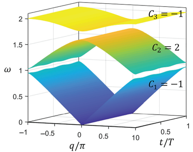
FIG. 2. Evolution of eigenfrequencies of an infinitely modulated lattice as a function of the nondimensional wavenumber and time with Chern numbers assigned to each band.
