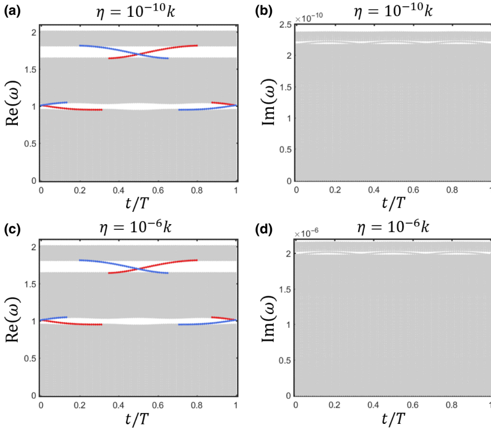
FIG. 8. Evolution of eigenfrequencies of a finite periodic lattice (300 masses) with different damping coefficients over one period of modulation under free boundary conditions. The real parts (a) and the imaginary parts (b) of the eigenfrequencies when \eta = 10^{-10}k ; The real parts (c) and the imaginary parts (d) of the eigenfrequencies when \eta = 10^{-6}k . Left and right edge modes are highlighted by blue and red circles, respectively.
