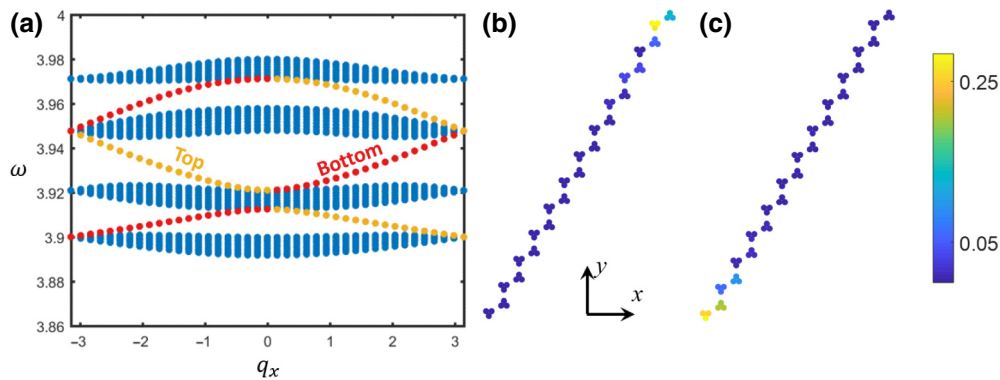
FIG. 14. (a) Bulk and edge spectra for a supercell of 12 unit cells under free boundary conditions at the top and bottom and periodic boundary conditions in the x direction. Bulk modes are shown by blue dots. Top (bottom) edge modes are shown by yellow (red) dots; (b),(c) Mode profiles of the one-way edge mode localized at the top and bottom of the supercell, respectively, corresponding to the frequency \omega = 3.93 .
