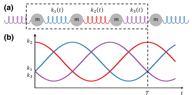
FIG. 1. A modulated 3-periodic spring-mass lattice: (a) Geometry; a unit cell is framed with dashed lines. (b) Time profiles of the modulated spring constants.
