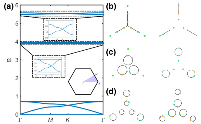
FIG. 10. (a) Dispersion diagrams for nonmodulated hexagonal lattices (insets show zoomed view). At \delta k = 0 , there are three degenerate points at K . The mass trajectories of the degenerate eigenstates are illustrated in (b) \omega = 5.52 , (c) \omega = 3.91 , and (d) \omega = 0.49 , respectively. A yellow dot corresponds to the initial position of the mass and a green dot corresponds to the position at a later small time.
