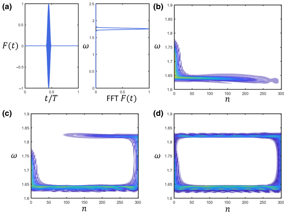
FIG. 6. (a) The transient force loading F in time and frequency domains; (b–d) The FFT of the wave field is taken at t=T, 2T , and 3T , respectively, illustrated as a one-way edge state in the (n, \omega) space.
