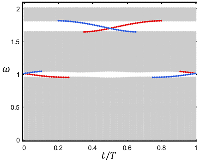
FIG. 4. Evolution of eigenfrequencies of a finite periodic lattice (300 masses) over one period of modulation under free boundary conditions. Two band gaps are visible and are traversed by the eigenfrequencies of edge states. The shaded gray regions indicate the bulk pass bands. Left and right edge modes are highlighted by blue and red circles, respectively.
