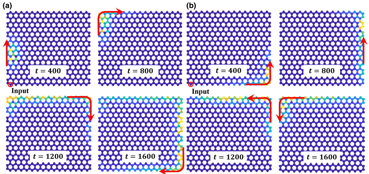
FIG. 16. Snapshots of one-way transmission of topological edge states with no backscattering at corners: (a) snapshots of the displacement amplitude as a color map for \{\phi_1, \phi_2, \phi_3\} = \{0, 2\pi/3, 4\pi/3\} at t = 400, t = 800, t = 1200, and t = 1600, respectively; (b) snapshots of the displacement amplitude as a color map for \{\phi_1, \phi_2, \phi_3\} = \{4\pi/3, 2\pi/3, 0\} at t = 400, t = 800, t = 1200, and t = 1600, respectively.
