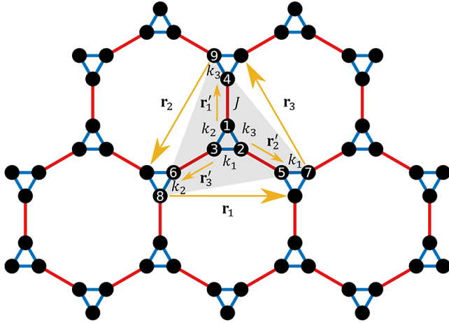
FIG. 9. A hexagonal lattice of modulated trimers composed of three interconnected masses coupled with each other by modulated springs (blue edges). Edges are massless springs and black nodes are massive perfect hinges. The spring stiffness k_j = k + \delta k \cos(\nu t + \phi_j) in trimers is periodically modulated in time at a frequency \nu and with amplitude \delta k in a rotation fashion. The red edges show the nearest springs with constant J between modulated trimers. A unit cell is highlighted.
