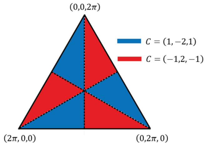
FIG. 3. Phase diagram of the 1D modulated lattice illustrating Chern numbers as a function of phase delays \{\phi_1, \phi_2, \phi_3\} interpreted as barycentric coordinates in the planes (\phi_1 + \phi_2 + \phi_3 = 2\pi) . Chern numbers are not defined over the dashed lines where degeneracies occur.
