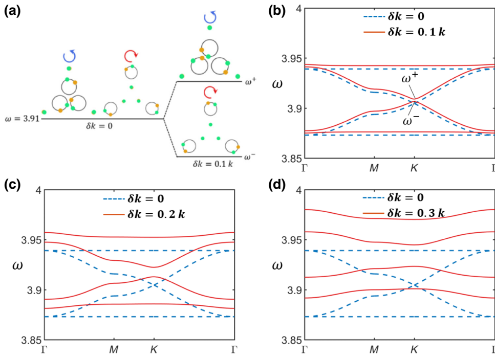
FIG. 11. (a) The modes split at \omega = 3.91 due to angular momentum bias with modulation amplitude \delta k = 0.1k . The dispersion curves of nonmodulated (blue dashed curves, \delta k = 0 ) and modulated hexagonal lattices [ \delta k = 0.1k in (b), 0.2k in (c), and 0.3k in (d)]. Note that only four bands of interest are shown and the time modulation has the effect of folding the dispersion curves along the frequency axis.
