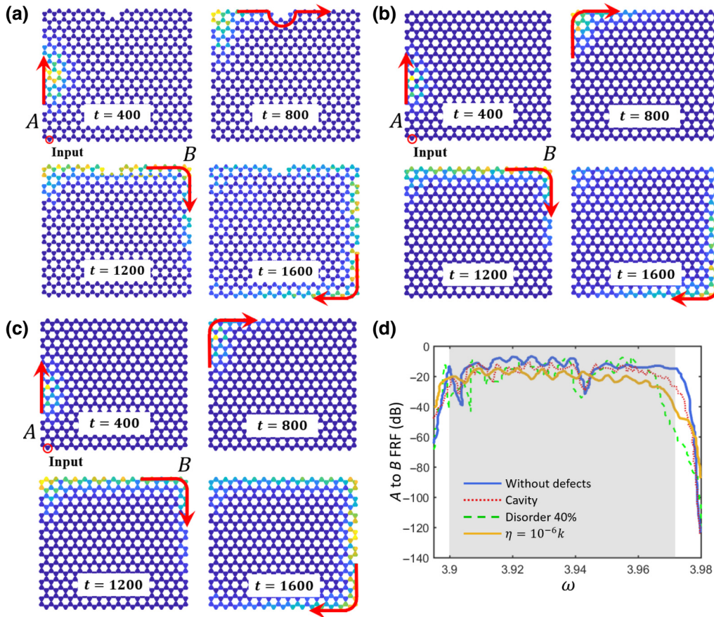
FIG. 17. Robustness demonstration of one-way transmission of topological edge states: (a) snapshots of the displacement amplitude with a cavity for \{\phi_1, \phi_2, \phi_3\} = \{0, 2\pi/3, 4\pi/3\} at t=400 , t=800 , t=1200 , and (4) t=1600 , respectively; (b) Snapshots of the displacement amplitude with 40% modulation disorders at t=400 , t=800 , t=1200 , and (4) t=1600 , respectively; (c) Snapshots of the displacement amplitude with the damping coefficient \eta = 10^{-6}k , at t=400 , t=800 , t=1200 , and (4) t=1600 , respectively; (d) Frequency response functions for the one-way topological edge states with defects and without defects for the frequency range of interest. The blue solid curve corresponds to the case without any defects while the red dotted, green dashed, and yellow solid curves correspond to the cases with a cavity, random modulation disorders, and dissipation effects, respectively.
