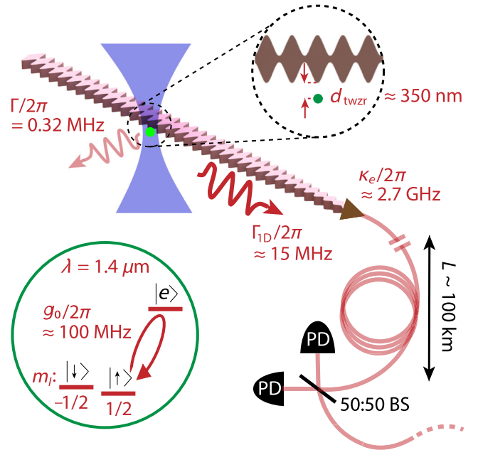
FIG. 1. Schematic overview. Silicon photonic crystal cavity with an ^{171}\text{Yb} atom trapped nearby in an optical tweezer. The minimum atom-device separation d_{\text{twzr}} \approx 350 \text{ nm} allowed by our approach corresponds to an atom-cavity system on a strong telecom-band transition with vacuum Rabi frequency g_0/2\pi \approx 100 \text{ MHz} and emission bandwidth of \Gamma_{\text{ID}}/2\pi \approx 15 \text{ MHz} , for a partially open cavity with external coupling \kappa_e/2\pi \approx 2.7 \text{ GHz} and atomic free-space linewidth of \Gamma/2\pi = 0.32 \text{ MHz} . The nuclear spin projections m_I are of the I = 1/2 nuclear spin of ^{171}\text{Yb} . The photon in the cavity is coupled to an optical fiber with length L \sim 100 \text{ km} . This system constitutes a node in a telecom quantum repeater in which entanglement between nodes is established by a Bell state measurement using a 50:50 beam splitter (BS) and single-photon detectors (PD).
