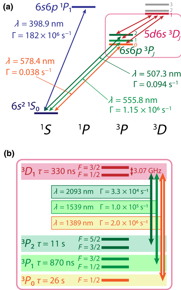
FIG. 2. Level diagram of the relevant states of ^{171}\text{Yb} . (a) Low-lying states of Yb in the singlet and triplet manifolds. The telecom transitions from the metastable 6s6p 3P_J states to the 5d6s 3D_1 state are highlighted in the red box. (b) Enlargement of the highlighted transitions. The nuclear spin in ^{171}\text{Yb} is I = 1/2 , so the hyperfine states are given by F = 1/2 when J = 0 and F = \{J + 1/2, J - 1/2\} when J \geq 1 . The lifetimes of the 3P_J states, transition wavelengths, and transition linewidths, as well as the lifetime and hyperfine splitting of the 3D_1 state, are given. We employ the transition shown with the orange double arrow.
