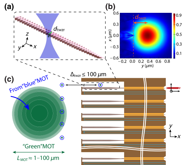
FIG. 5. Coupling an Yb atom to a silicon photonic crystal cavity via an optical tweezer trap. (a) An enlargement illustrating the atom in a tweezer near the device at a distance d_{\text{twzr}} . (b) The electric field magnitude of the tweezer trap in arbitrary units at a distance of d_{\text{twzr}} = 350 nm from the edge of the device. (c) Schematic of the silicon chip. The silicon top layer is brown and the insulator layer below is orange. The blue microstrips on the chip are used for Ohmic temperature control and applying rf magnetic fields. The lensed fiber on the right can be coupled to any cavity using a three-dimensional (3D) translation stage. Wavy white lines indicate cuts to show the entire chip. The green circle on the left is the Yb MOT. Atoms can be shuffled between it and the device using optical tweezers. This architecture allows simultaneous operation of multiple Yb-cavity nodes on a single device.
