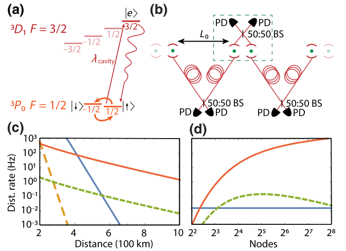
FIG. 3. Spin-photon entanglement scheme and quantum repeater operation. (a) The relevant (irrelevant) hyperfine states are shown in solid (semitransparent) colors. The cavity-enhanced transition wavelength is \lambda_{\text{cavity}} . (b) A single trapped ^{171}\text{Yb} atom in a cavity is represented by a green dot inside two curved semicircles. Local node pairs are shown in the dashed box. Node pairs are separated by L_0 . BS denotes the beam splitter and PD the single-photon detector. (c) The entanglement distribution rate versus total distance via direct communication at 10 GHz for 1550 nm (solid blue curve) and 1390 nm (large-dashed orange) and via a quantum repeater with 2^4 nodes with (without) local deterministic entanglement, shown as a solid red (short-dashed green) curve. Note that a 10-GHz rate for the direct transmission scheme [62] can be interpreted as an information-theoretic bound for information distribution without quantum repeaters if an ideal single-photon source with a 10/1.44 = 6.9 -GHz repetition rate is employed [63]. (d) The entanglement distribution rate over 600 km versus the number of nodes via direct communication at 10 GHz for 1550 nm (solid blue) and 1390 nm (large-dashed orange, not visible) and via a quantum repeater with (without) local deterministic entanglement, shown as a solid red (short-dashed green) curve.
