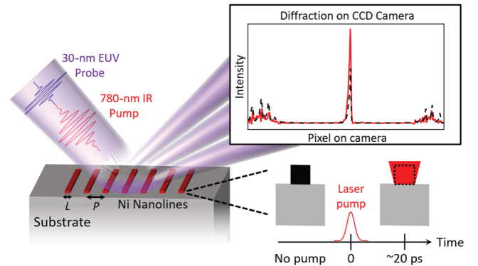
FIG. 1. EUV thermal and acoustic nanometrology. Gratings of nickel nanolines of linewidth L and period P are fabricated on silicon and fused-silica substrates. An ultrafast IR laser pulse heats the nanolines and they impulsively thermally expand (shown in lower right). An ultrafast EUV pulse then probes the sample as a function of time delay by measuring diffracted light using a CCD camera. The diffraction efficiency for a thermally excited sample (red in inset) changes compared to an unperturbed sample (black dotted line in inset). This change in diffraction efficiency captures the thermal and elastic dynamics that are deforming the sample surface. Note the change in the diffraction pattern shown is magnified 150 \times for illustration purposes.
