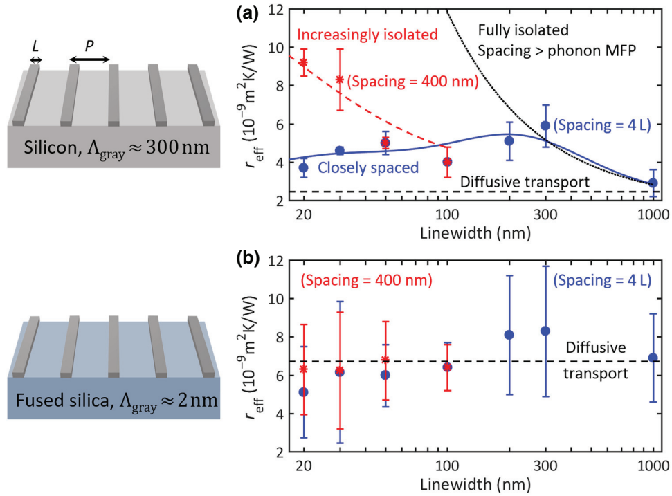
FIG. 3. Best fit effective thermal-boundary resistivity for nanolines on silicon and fused silica. (a) For silicon (gray MFP \approx 300 nm [12,21]), as the linewidth is reduced below 50 nm, the effective resistivity of the constant 25% duty cycle gratings (blue points) decreases, which is a return toward the diffusive prediction (thin-film case, black dashed line). In contrast, the constant 400-nm-period gratings' resistivities increase as the linewidth is reduced (red points), mapping the transition from dominant collective effects toward isolated quasiballistic thermal transport (isolated prediction, black dotted line). The blue solid line is the 25% duty cycle collectively diffusive prediction from [12], whereas the red dashed line is a fit with the same model to the new data. (b) For fused silica, the resistivities of constant duty cycle (blue points) and 400-nm-period (red points) gratings all agree within error bars. This indicates that there is no nondiffusive transport that depends on experimental geometry for this short-phonon MFP material (approximately 2 nm [15]), and that there are no dominant systematic errors coming from the grating geometry independent of the sample substrate material. The dotted line is the average of all grating resistivities on fused silica (6.7 nK m 2 /W). Error bars in (a) and (b) are calculated by the standard deviation of best fit values from multiple measurements.
