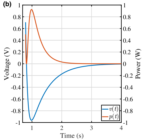
FIG. 6. (a) The corresponding RLC circuit after the stopping of temporal modulation. (b) The instantaneous voltage and the power consumed by the resistance R = 1 \Omega . Here t_0 = \pi/4\omega , \omega = 1 \text{ rad/s} , R_0 = 1 \Omega , A = 1 \text{ V} , and I_0 = 1 \text{ A/s} .
