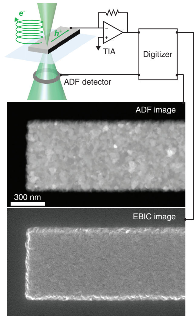
FIG. 1. STEM SEEBIC imaging of a metal electrode. (top) A cartoon representation of the basic setup shows the electron beam rastering over a bare Al electrode. Scattered electrons produce the usual ADF image (middle). SEs ejected from the electrode leave holes behind, producing a positive current and corresponding bright contrast in the EBIC image (bottom). The imaged electrode is maintained at virtual ground by the TIA.
