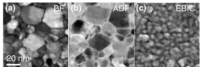
FIG. 5. Conventional STEM and STEM SEEBIC images of metallic grains in a Ti/Pt film. Simultaneously acquired BF (a), ADF (b), and EBIC (c) images of a Ti(5 nm)/Pt(25 nm) electrode on a Si 3 N 4 membrane.
