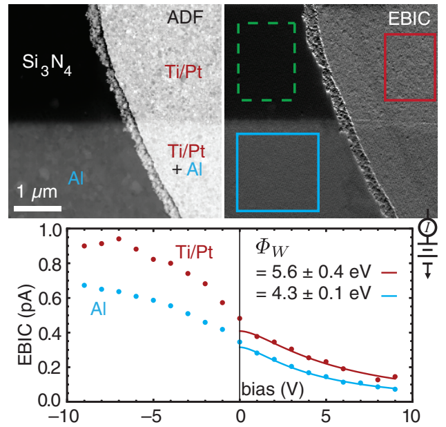
FIG. 4. ADF and EBIC images of Ti/Pt and Al electrodes and average SEEBIC from each material vs electrode bias. The images show four different material combinations: the bare Si 3 N 4 membrane, Ti(5 nm)/Pt(25 nm), 100-nm Al, and Ti(5 nm)/Pt(25 nm)/Al(100 nm). The plot shows the average signal in the SEEBIC image measured on Al (blue box) and Ti/Pt (red box), with the average current measured on Si 3 N 4 (green box) subtracted, for each bias value. The solid lines are fits to the SE-emission-current equation [Eq. (2)] for V > 0 , with the work functions and zero-bias currents as free parameters.
