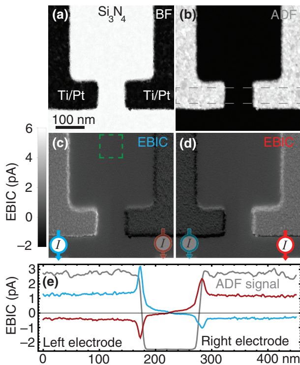
FIG. 2. Conventional STEM and double STEM SEEBIC imaging of Ti/Pt electrodes. The simultaneously acquired (a) BF, (b) ADF, and (c),(d) STEM EBIC images show Ti(5 nm)/Pt(25 nm) electrodes on a Si 3 N 4 membrane. TIAs are connected to the electrodes as indicated by the blue and red symbols in the STEM EBIC images, with the symbol shown as opaque in the image generated by that TIA. Bright (dark) contrast corresponds to positive (negative) current, as indicated by the current scale for (c) and (d) that is to the left of (c). The gray, blue, and red plots in (e) show line profiles from (b)–(d) taken in the region indicated by the gray rectangle in (b). The gray plot is in arbitrary units and the blue and red plots use the scale on the y axis. The images in (a)–(d) are rotated 90° counterclockwise, so that the fast scan direction is bottom to top. EBIC values in (c),(d) are given relative to their respective averages from the region outlined in green in (c).
