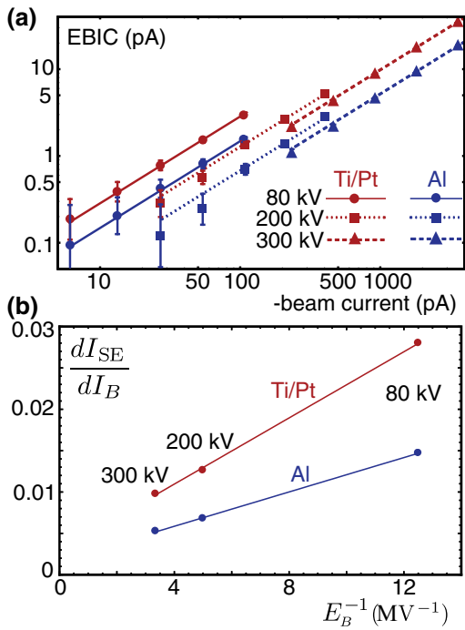
FIG. 3. EBIC vs beam current and SE yield vs inverse beam energy. In the plot (a), the EBIC current from Ti(5 nm)/Pt(25 nm) and 100-nm Al electrodes is shown (with fits to I_{SE} = \delta \times I_B ) for five different beam currents I_B at each accelerating voltage of 80, 200, and 300 kV. The EBIC uncertainty is taken to be 0.1 pA. In the plot (b), the SE yield \delta for each material, determined from the six fits in the plot (a), is linear in E_B^{-1} , as predicted by Eq. (2).
