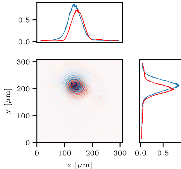
FIG. 32. Experimental measurement, the first laser pass (blue) and last pass (red) measured at the IP by the IIOS.
