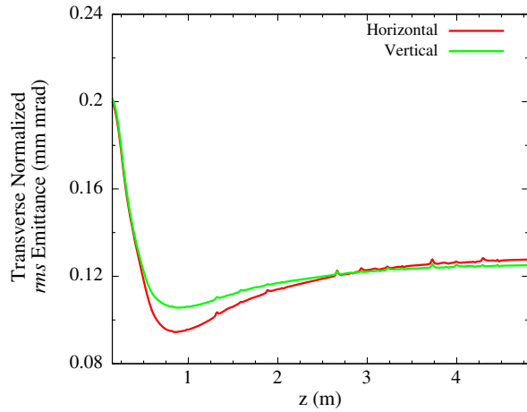
FIG. 10. Transverse normalized rms emittances of the bunch off the cathode tracked through an unoptimized version of the accelerating section as a function of the longitudinal position.
