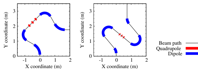
FIG. 3. Basic layout examples of 3\pi (left) and 4\pi (right) bunch compressors. Beam enters at (0, 0).
