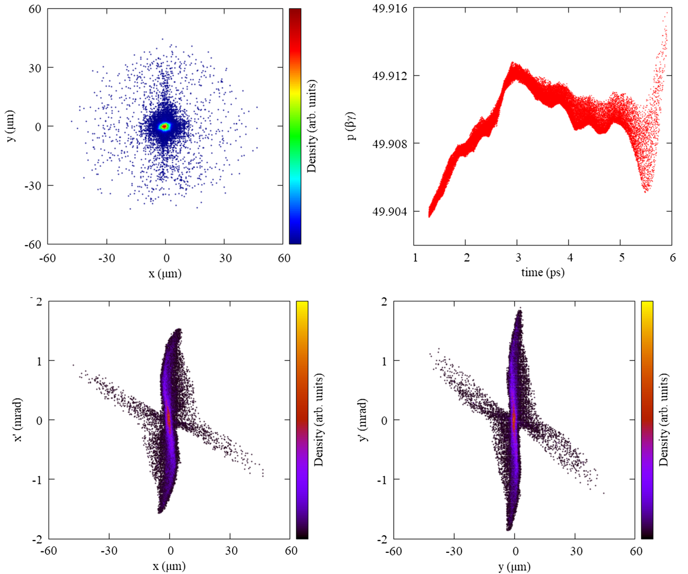
FIG. 12. Beam spot (top left), longitudinal phase space (top right), horizontal phase space (bottom left), and vertical phase space (bottom right) of the electron bunch at the IP.
