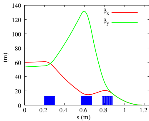
FIG. 11. \beta_x and \beta_y as a function of s in the final focusing section of the design. The locations of the three quadrupoles are shown along the horizontal axis.
