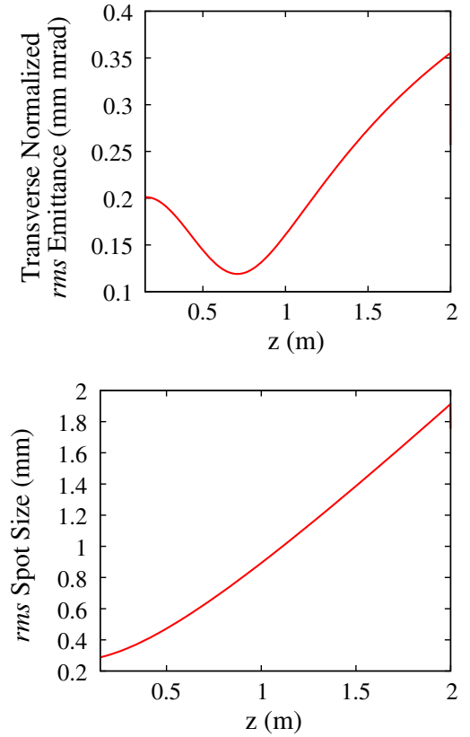
FIG. 9. Transverse normalized rms radial emittance (top) and transverse spot size (bottom) of bunch drifting after gun exit as a function of longitudinal position.
