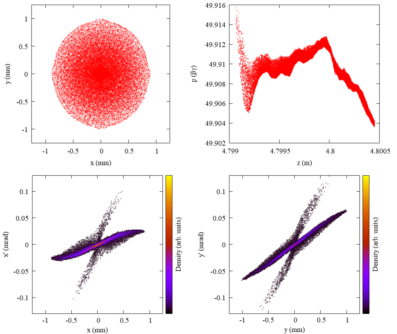
FIG. 7. Beam spot (upper left), longitudinal phase space (upper right), horizontal phase space (bottom left), and vertical phase space (bottom right) of bunch after exiting the linac.
