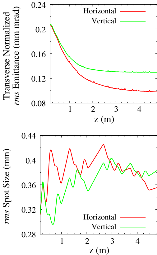
FIG. 8. Transverse normalized rms emittances (top) and spot sizes (bottom) of bunch passing through the linac.
