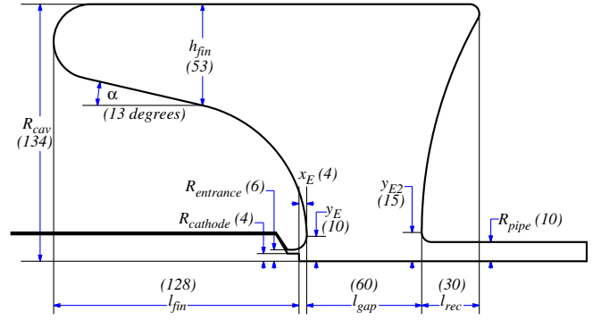
FIG. 4. Diagram of gun geometry with parameters and quantities. Quantities are rounded to the nearest millimeter and given in millimeters, except where explicitly indicated.
