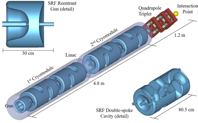
FIG. 1. A schematic of the entire design. The first cryomodule contains the gun and two double-spoke cavities, the second contains the last two double-spoke cavities. Three quadrupole magnets follow the linac, before the interaction point. Detailed images of the gun and the double-spoke cavity are shown in the top left and bottom right, respectively.
