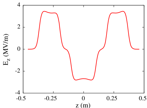
FIG. 6. The accelerating electric field along the beamline of the double-spoke SRF cavity.
