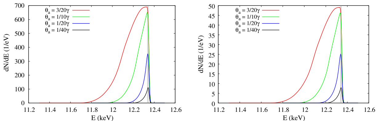
FIG. 14. Number spectra for different apertures generated using 4 000 particles for a 3.2 \mu\text{m} laser spot size (left) and a 12 \mu\text{m} laser spot size (right). Grey box indicates 0.1% bandwidth. Suggested apertures for brilliance calculation only.
