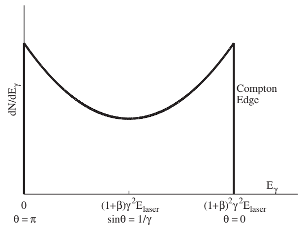
FIG. 2. Number density of scattered photons as a function of the energy of scattered photons. Annotated Fig. 2 from [5].
