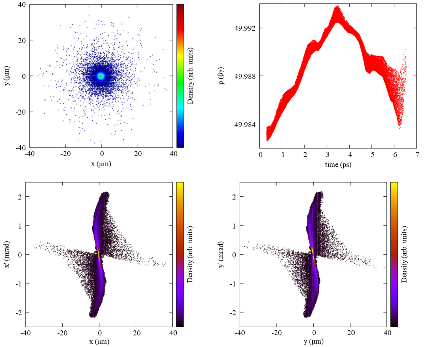
FIG. 13. Beam spot (top left), longitudinal phase space (top right), horizontal phase space (bottom left) and vertical phase space (bottom right) of the electron bunch at the IP, using elliptical cavities in the linac.
