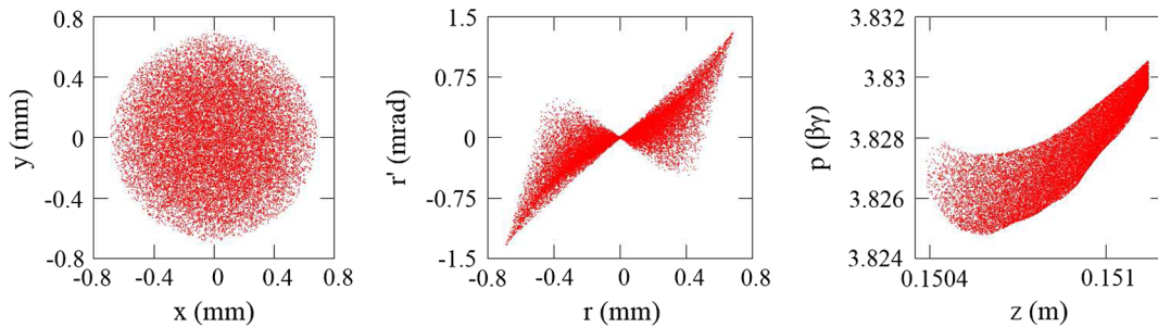
FIG. 5. Beam spot (left), transverse phase space (center), and longitudinal phase space (left) of bunch exiting gun.
