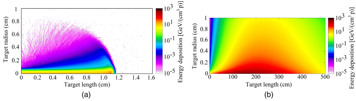
FIG. 11. Two-dimensional energy deposition in units of \text{GeV}/\text{cm}^3 per proton in a solid graphite target at the energies of (a) 50 MeV and (b) 50 TeV. The rms beam size is \sigma = 0.2 mm.
