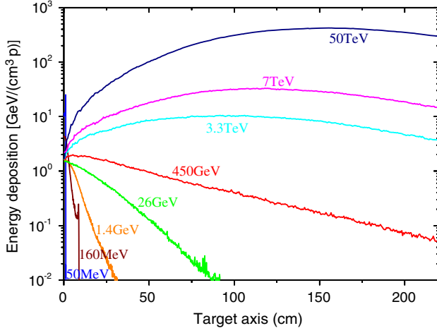
FIG. 14. Energy deposition per incident proton as a function of the depth into the solid graphite target at r = 0 . The beam size is 0.2 mm for all the presented energies from 50 MeV to 50 TeV.
