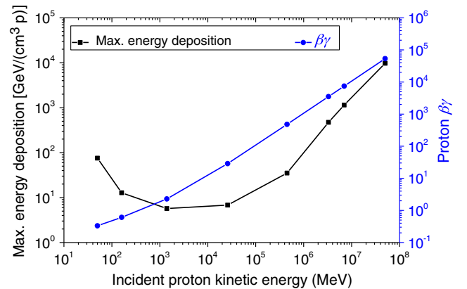
FIG. 6. Maximum energy deposition in copper as a function of the incident proton kinetic energy. The corresponding values of \beta\gamma are plotted as well. The beam size is constant (0.2 mm) for the energies from 50 MeV to 50 TeV.
