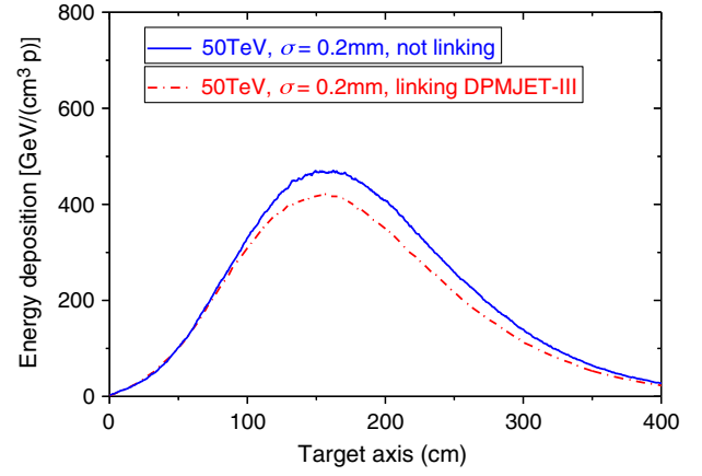
FIG. 16. Energy deposition of 50 TeV proton in graphite along the target axis with and without linking FLUKA and DPMJET-III. Without linking, the maximum energy deposition is 11% higher than that for the case of linking.
