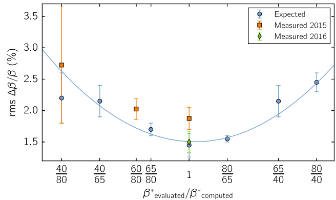
FIG. 11. The rms \beta -beating when calculating a correction at a certain \beta^* and applying it at a different. The blue points are based on simulations while the green and orange are based on measurements.
