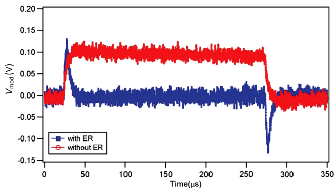
FIG. 19. Forward power drive signal for an SRF cavity with 250 \mu sec-duration tune beam with single beam (red) and a two-beam, energy recovering setup (blue) (from [93]).
