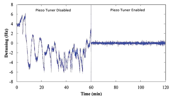
FIG. 31. Piezotuner control off and on (from [157]).
