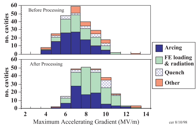
FIG. 13. Cavity performance improvement with helium processing 1996–1998 (from [85]).
