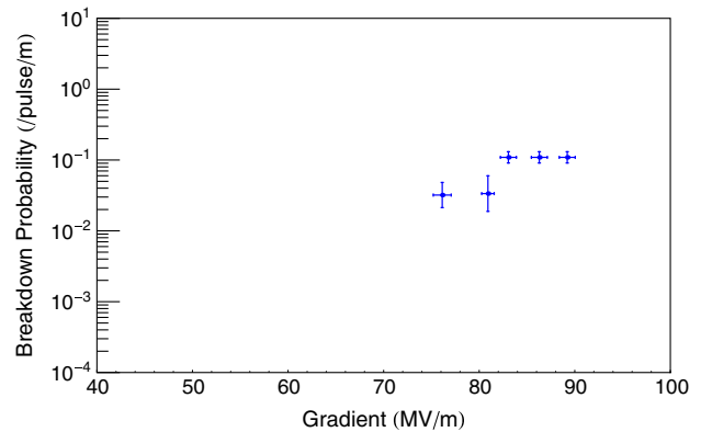
FIG. 25. Breakdown probability as a function of gradient for the PBG structure.
