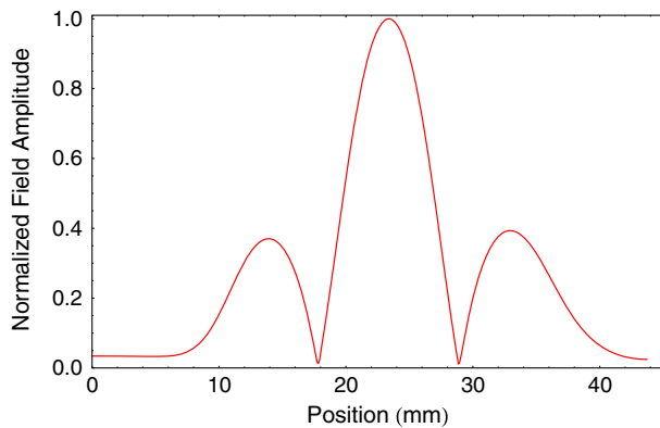
FIG. 5. Normalized profile of simulated electric field on axis in PBG structure; the field amplitude in each coupling cell is approximately half that in the PBG cell.
