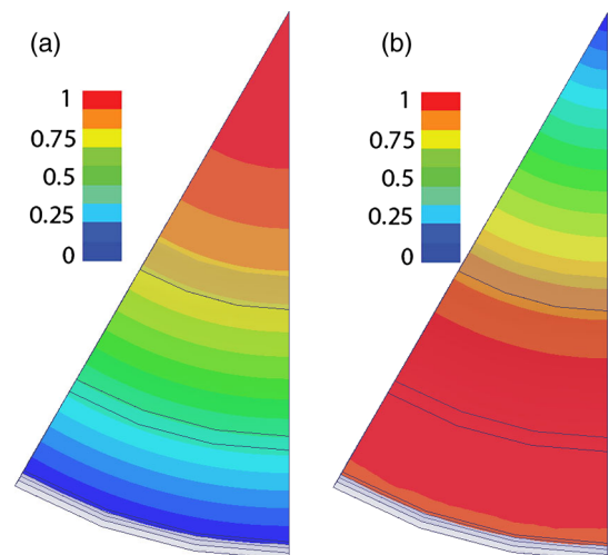
FIG. 12. Electric (a) and magnetic (b) field amplitudes looking at top-down view of a 30 degree section of the structure. The peak surface electric field of 197 MV/m for a 100 MV/m accelerating gradient from 2.0 MW of input power is seen on-axis. The peak surface magnetic field of 421 kA/m for an accelerating gradient of 100 MV/m is on the end plate of the structure.
