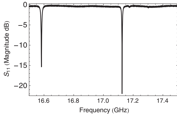
FIG. 16. S_{11} of DLWG structure showing resonances for the \pi/2 and \pi modes at increasing frequency.
