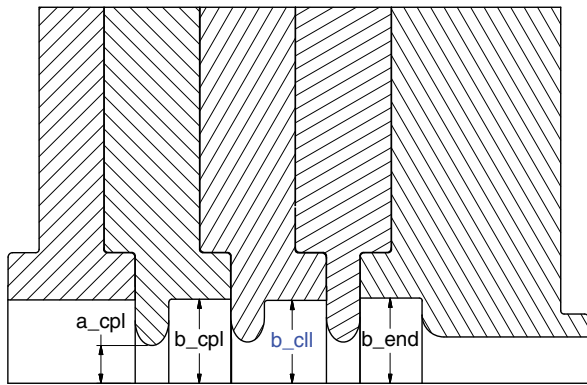
FIG. 8. Axisymmetric views of the assembly drawing of the 17.1 GHz MIT-DLWG structure showing the additional fixed parameters for the structure in black and the one tuning parameter in blue.
