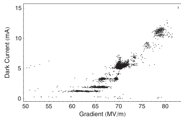
FIG. 20. Dark current in mA as a function of gradient in MV/m for one day of testing of MIT-DLWG structure. A representative sampling of the data is shown.
