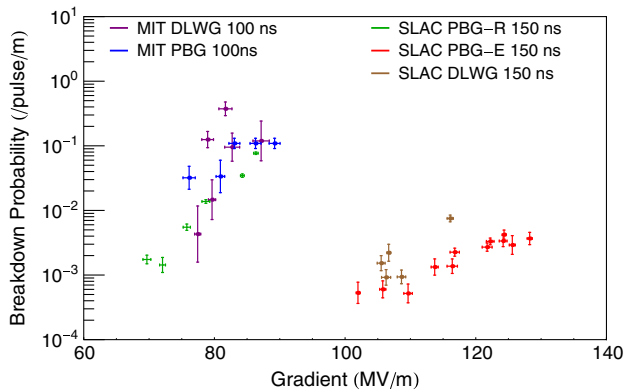
FIG. 26. Breakdown probability as a function of gradient for MIT-PBG, MIT-DLWG, SLAC PBG-R, SLAC PBG-E, and SLAC DLWG structures. For the MIT-DLWG structure only data after the return to high-gradient operation in Phase 2 is shown.
