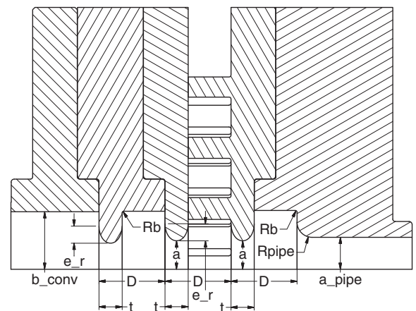
FIG. 2. Axisymmetric views of the assembly drawing of the 17.1 GHz PBG structure showing the fixed parameters of the structures. The five plates that are defined in the drawing correspond to the five copper-colored elements shown in Fig. 1.
