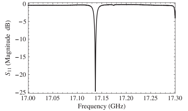
FIG. 22. S_{11} of the PBG structure showing resonance for the \pi mode.
