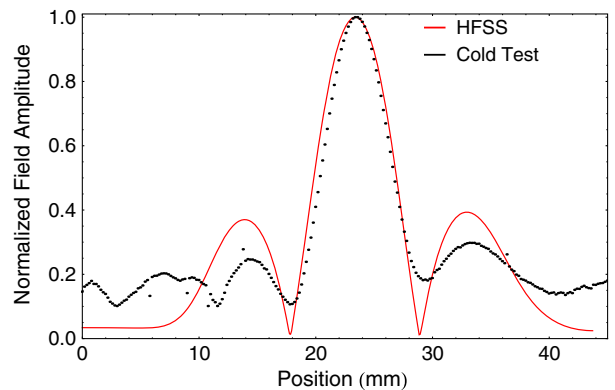
FIG. 23. Comparison of the simulated and measured axial field profiles for the \pi mode of the PBG structure.
