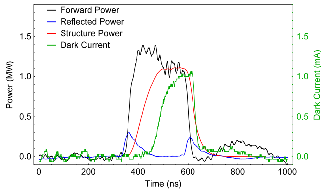
FIG. 14. Sample forward power, black, reflected power, blue, downstream current monitor, green, and calculated structure power, red, traces are shown. This trace was recorded during operation of the pre-test structure, and represents a gradient of 67 MV/m in the PBG structure.
