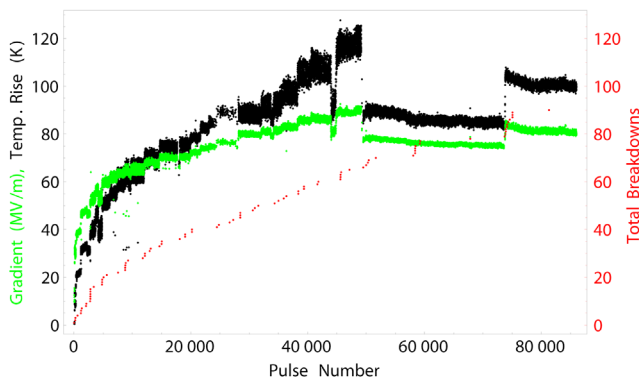
FIG. 24. Summarized results showing the gradient (green), temperature rise (black), and total number of breakdowns (red) for the PBG testing. Note the extremely low breakdown rate even during initial processing.
