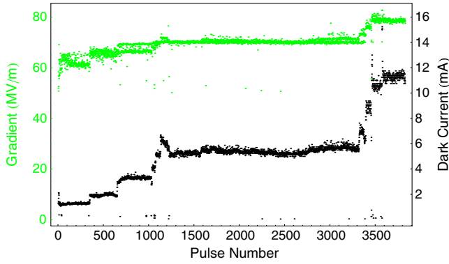
FIG. 21. Dark current in mA and gradient in MV/m as a function of pulse number for a representative sampling from one day of testing of DLWG structure.
