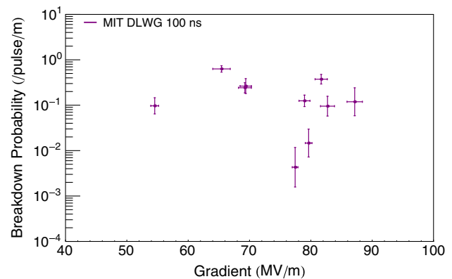
FIG. 19. Breakdown probability as a function of gradient for the DLWG structure.
