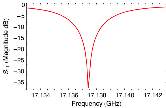
FIG. 4. Calculated reflection as a function of frequency for the 17.1 GHz PBG structure.
