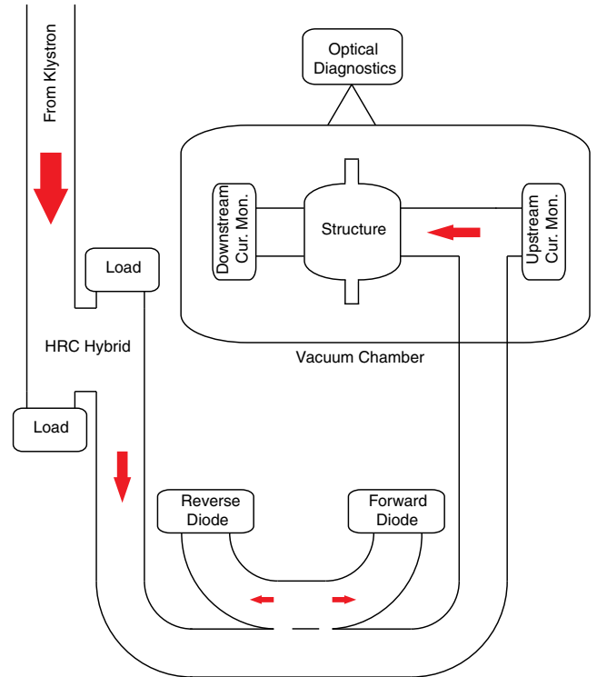
FIG. 13. A schematic view of the MIT standing-wave test stand and associated diagnostics is shown. Power is coupled from the klystron through a 4.4 dB hybrid made by Haimson Research Corporation (HRC) before coupling into the structure. Incident and reflect rf power signals are measured using diode detectors on a 65 dB waveguide directional coupler. Upstream and downstream current monitors are present within the vacuum chamber.
