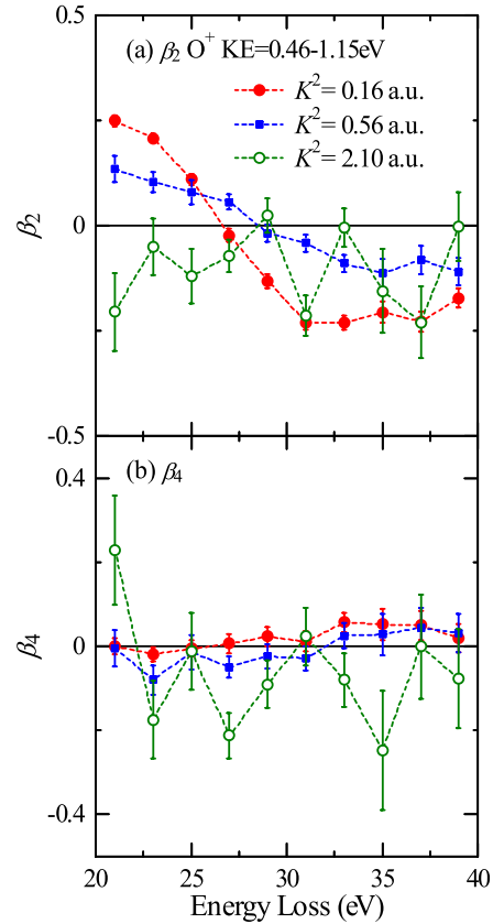
FIG. 5. Generalized asymmetry parameters, (a) \beta_2 and (b) \beta_4 , for the B^2\Sigma_g^- ionization at K^2 = 0.16, 0.56, and 2.10 \text{ a.u.} Dashed lines are drawn as a guide for the eye.
