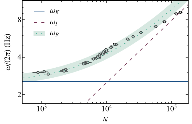
FIG. 2. Angular frequency of the lowest axial mode as a function of atom number, N . \omega_K is the mode frequency in an ideal gas, and \omega_I is the frequency of Bogoliubov sound with speed (gn/m)^{1/2} and wavelength 2L . These calculations use trap dimensions L = 26 \mu\text{m} and R = 16 \mu\text{m} . The shaded band \omega_B shows the results of numerical Bogoliubov diagonalization (see Sec. III B) accounting for the uncertainty of \pm 1 \mu\text{m} in L and R .
