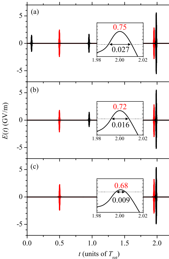
FIG. 5. Optimally designed Gaussian subpulses in the (a) quintuple-pulse control, (b) quadruple-pulse control, and (c) triple-pulse control schemes. Each inset shows a magnified view of the time evolution of the averaged degree of alignment in which the maximum value is given. The horizontal dashed lines specify 0.67, which is the maximum averaged degree of alignment achieved by a pair of optimal double Gaussian subpulses with the total fluence of 1.3\text{J}/\text{cm}^2 . The period (units of T_{\text{rot}} ) during which the averaged degree of alignment is larger than 0.67 is also shown in each inset.
