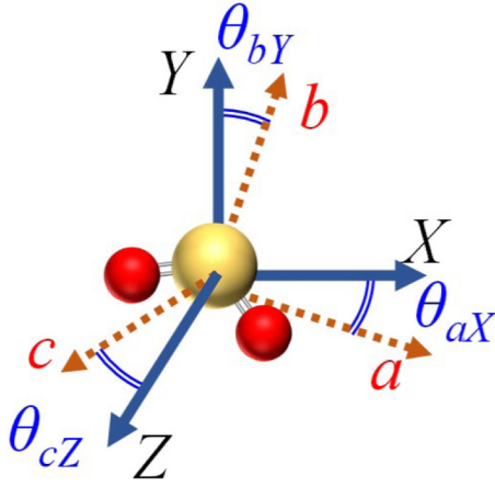
FIG. 1. Molecule-fixed a , b , and c axes of \text{SO}_2 and space-fixed X , Y , and Z axes. Three of the angles between the molecule-fixed axes and the space-fixed axes are shown.
