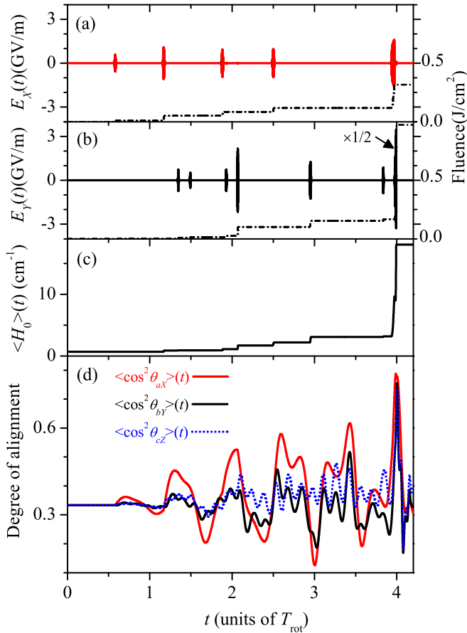
FIG. 2. Results of optimization control simulation with the final time, t_f = 4.0 , in units of T_{\text{rot}} when the a and b axes are chosen as the target axes. Optimized (a) X and (b) Y components of the laser field. Dot-dashed lines indicate fluence as a function of time. (c) Expectation value of the free rotational Hamiltonian, H_0 . (d) Red (gray) solid, black solid, and blue dashed lines represent the time evolution of the degrees of alignment, \langle \cos^2 \theta_{aX} \rangle(t) , \langle \cos^2 \theta_{bY} \rangle(t) , and \langle \cos^2 \theta_{cZ} \rangle(t) , respectively.
