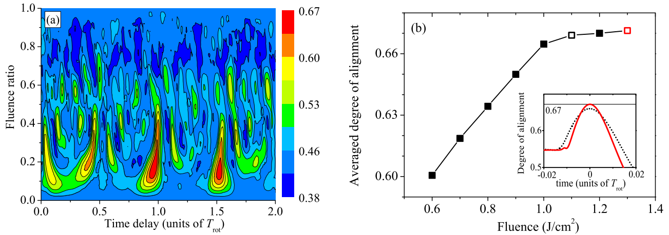
FIG. 4. (a) Contour plot of the largest averaged degrees of alignment achieved by mutually orthogonal, linearly polarized Gaussian subpulses (see text) as a function of delay time (horizontal axis) and fluence ratio (vertical axis). As we consider all possible combinations of the target molecular axes with respect to the space-fixed axes, the X subpulse is assumed to appear before the Y subpulse. Fluence ratio is defined by the X -subpulse fluence divided by the total fluence. (b) Maximum averaged degree of alignment as a function of total fluence. The values when the total fluence is 1.1 and 1.3 J/cm 2 are specified by black and red (gray) open squares, respectively. Red solid and black dashed lines in the inset, respectively, show a magnified view of the time evolution of the averaged degrees of alignment when the total fluence is 1.1 and 1.3 J/cm 2 . Each time when each averaged degree of alignment becomes a maximum is set to zero for illustrative purposes.
