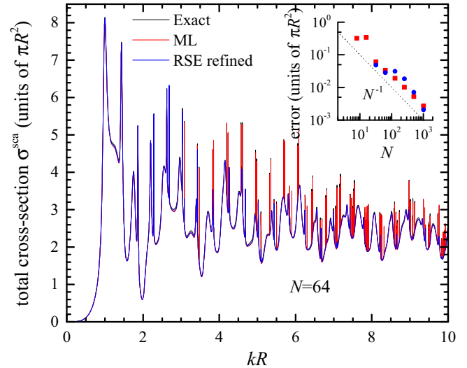
FIG. 10. Total scattering cross section \sigma^{\text{sca}}(k) for a dielectric sphere of \epsilon = 9 in vacuum. The analytical result using using Mie theory [33] (black) is compared with ML expansion for a basis size of N = 64 , using the exact RSs for \epsilon = 9 (red line), and the RSs determined by the RSE with refinement, using as basis a sphere with \epsilon = 4 (blue line). Inset: absolute error averaged over 0 \leq kR \leq 10 , as function of the basis size N . The dotted line gives N^{-1} .
