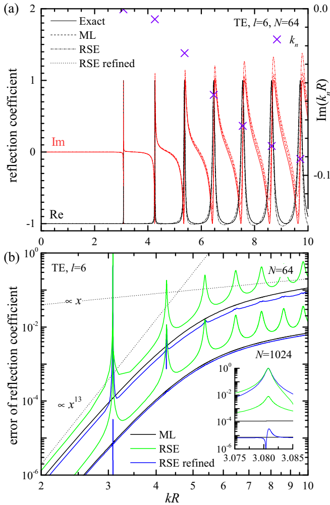
FIG. 3. As Fig. 2, but for l = 6 . The inset in (b) is a zoom around the fundamental WG RS.
