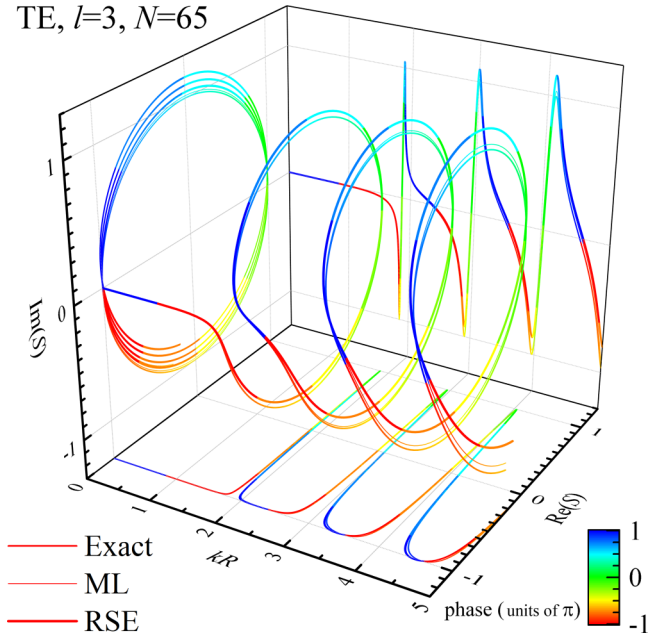
FIG. 1. Complex reflection coefficient S_{lmp}^{imp}(k) for TE polarization ( p = \text{TE} ) and l = 3 for a dielectric sphere of \epsilon = 9 in vacuum. The exact analytic result (normal line) is compared with the ML expansion using the exact RSs for \epsilon = 9 (thin line) and with the RSE calculation using a basis sphere of \epsilon = 4 (thick line), both computed for a basis size of N = 65 . 3D representation with the phase given by the line color.
