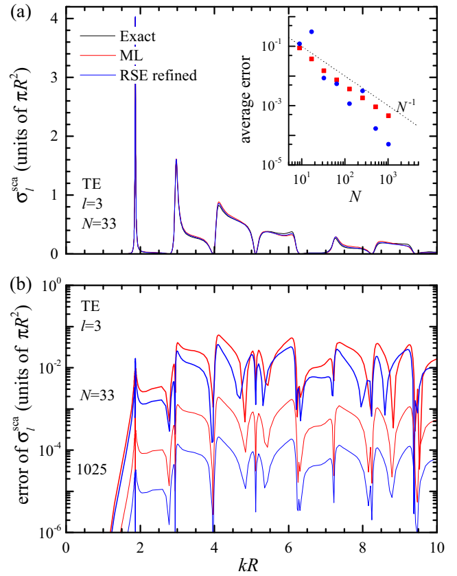
FIG. 6. (a) Partial scattering cross section \sigma_l^{\text{sca}}(k) for TE polarization and l = 3 for a dielectric sphere of \epsilon = 9 in vacuum. The analytical result (black) is compared with the ML expansion for a basis size of N = 33 , using the exact RSs for \epsilon = 9 (red line), and the RSs determined by the RSE with refinement, using as basis a sphere with \epsilon = 4 (blue line). (b) Absolute error |\sigma_l^{\text{sca}}(k) - \sigma_l^{\text{sca}(\text{exact})}(k)| for ML (red line) and RSE calculation (blue line). Results for a basis size N = 33 are given as thick lines, and for N = 1025 as thin lines. Inset in (a): absolute error averaged over the range of 0 \leq kR \leq 10 , as function of the basis size N . The dotted line gives N^{-1} .
