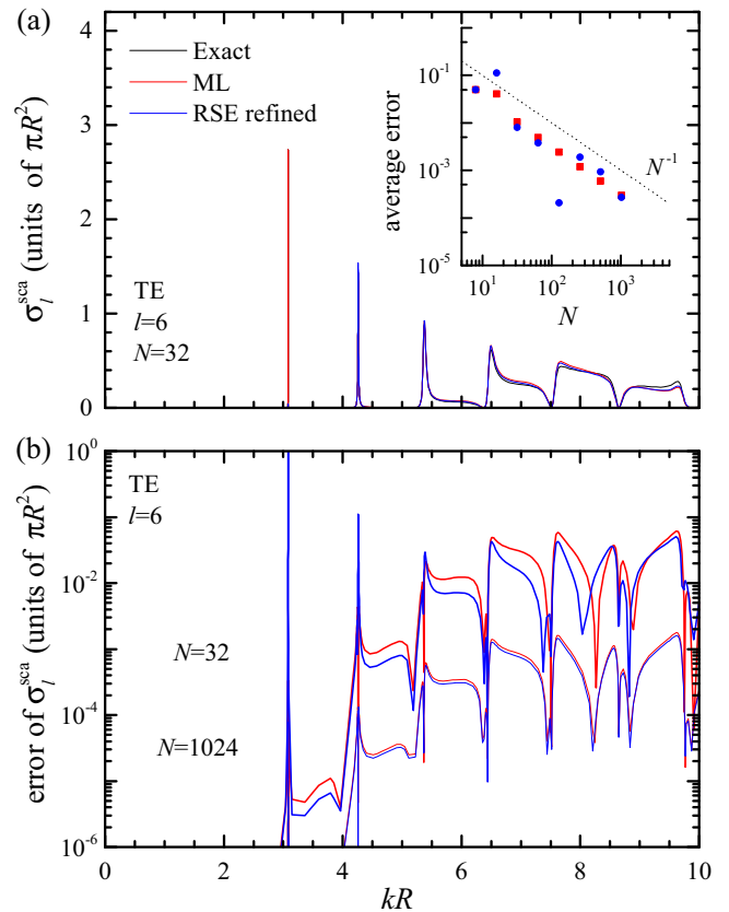
FIG. 8. As Fig. 6 but for l = 6 , and basis sizes N = 32 and 1024 as labeled.
