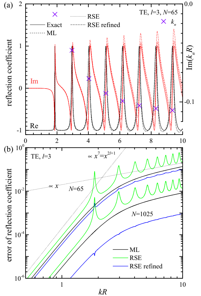
FIG. 2. (a) Complex reflection coefficient S_{lmp}^{imp}(k) for TE polarization ( p = \text{TE} ) and l = 3 for a dielectric sphere of \epsilon = 9 in vacuum. \text{Re}(S) in black, \text{Im}(S) in red. The analytical result (solid line) is compared with the ML expansion using the exact RSs for \epsilon = 9 (dashed line) and with the RSE calculation using a basis sphere of \epsilon = 4 (dashed-dotted line), both calculated for a RS basis size of N = 65 , and a refined RSE calculation including a first-order correction of the RS fields (dotted line). The RS wave numbers k_n are given as crosses. (b) Absolute error |S - S^{(\text{exact})}| of the ML (black solid line), the RSE (green solid line), and the refined RSE results (blue line). Results for basis sizes N = 65 and 1025 as labeled. The dotted lines show asymptotic power-law dependencies as labeled.
