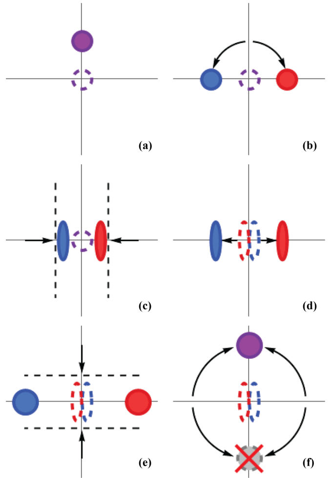
FIG. 4. Phase-space representation of the state of the system as it progresses through the apparatus shown in Fig. 3 for the case of \phi = \pi/2 . The horizontal axes correspond to the real part of the Wigner distribution or Q function as in Fig. 2, while the vertical axes correspond to the imaginary part. (a) The initial coherent state |\alpha_0\rangle (solid circle) along with the idler mode of the OPA (dotted circle) which is initially in its vacuum state. (b) Cat state created by the first single-photon interferometer, where the Kerr medium and a constant phase shift apply a net phase shift of \pm\pi/2 depending on the path taken by the single photon. (c) Reduced overall amplitude of the cat state components due to squeezing along the real axis. The squeezing also increases the amplitude along the imaginary axis. (d) Compensation for the effects of loss using a deterministic amplifier, which also displaces the idler modes. This results in a state where the signal and idler modes are entangled. (e) Restoration of the original amplitude of the cat state using antisqueezing. (f) A second phase shift of \pm\pi/2 is produced in the analyzer of Fig. 3, depending on the path taken by the second single photon. Postselecting on a net phase shift of zero results in an overlap between the two original components of the cat state. This gives quantum interference, the visibility of which provides a measure of the amount of decoherence, as described in more detail in Ref. [5].
