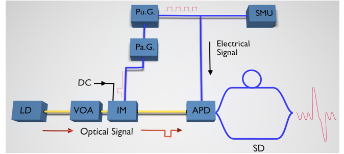
FIG. 2. Experimental setup. Pu.G.: pulse generator; Pa.G.: pattern generator; SMU: source measure unit; LD: laser diode; VOA: variable optical attenuator; IM: intensity modulator; APD: avalanche photodiode; SD: self-differencer.
