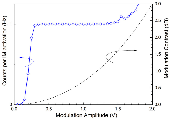
FIG. 5. APD counts per IM activation and IM contrast as a function of the ac signal driving the IM, for a constant incident optical power of 1 mW and a modulation pattern 1/128. We note that the APD discrimination level is deliberately set too high (26 mV) to enable blinding when the IM is switched off.
