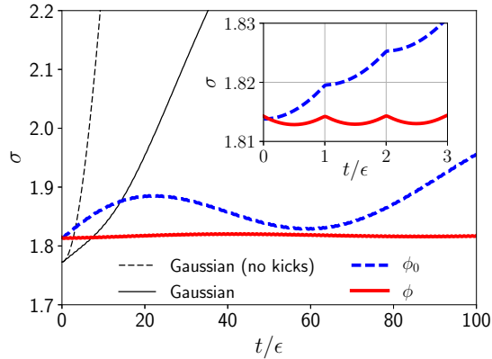
FIG. 3. Spatial width of \Psi(x,t) as a function of t for \epsilon = 0.5 and three different initial states: a Gaussian state (thin solid black curve), \phi_0(x) = \frac{1}{2}\text{sech}\frac{x}{2} (thick dashed blue curve), and \phi(x) from Eq. (21) (thick solid red curve). The thin dashed black curve corresponds to the free-space evolution of the Gaussian wave packet. Inset shows short time behavior.
