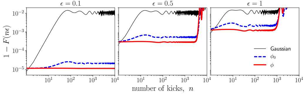
FIG. 2. Fidelity of stroboscopic solitons. Dependence of the fidelity error 1 - F(n\epsilon) on the number of kicks for different kicking strength \epsilon [see Eq. (4)]. Three different initial states are considered: a Gaussian state (thin solid black curves), \phi_0(x) = \frac{1}{2} \operatorname{sech} \frac{x}{2} (thick dashed blue curves), and \phi(x) approximated by Eq. (21) (thick solid red curves).
