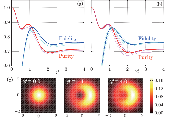
FIG. 6. (a, b) Time evolution of the fidelity F(t) = \langle 1|\rho(t)|1\rangle and the purity P(t) = \text{Tr}[\rho(t)^2] ; the solid red and blue lines are the case of ideal setup, while cyan and magenta lines are the case under (a) decoherence and (b) parameter mismatch. (c) Q function of the system state at \gamma t = 0, 1.1, 4.0 in the ideal setting.
