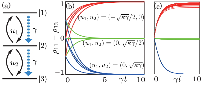
FIG. 4. (a) Energy diagram of the states and time evolution of \rho_{11} - \rho_{33} in the case \kappa = 100\gamma , (b) with several initial states in the ideal setup and (c) with a specific initial state in the realistic setup.
