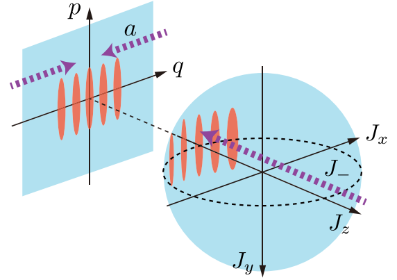
FIG. 5. Projection of the spin operators to the boson operators, for a large atomic ensemble.
