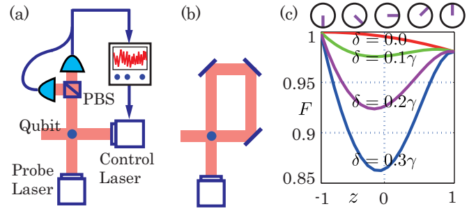
FIG. 3. (a) MF and (b) CF configuration for qubit control. (c) Fidelity F = \langle \psi | \rho(\infty) | \psi \rangle between the ideal target state |\psi\rangle and the steady state \rho(\infty) in the realistic model.
