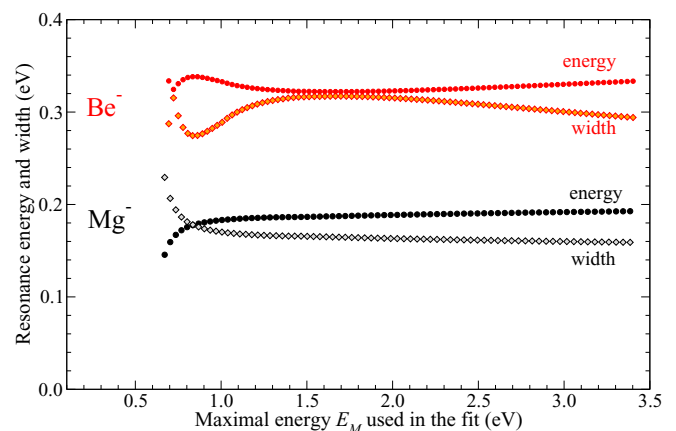
FIG. 2. Resonance energy (shown as circles) and width (displayed as diamonds) calculated for Be - and Mg - as functions of the energy extent defined by the maximal energy E_M . The exponents \gamma are fixed at \gamma = 0.035 for Be - and \gamma = 0.025 for Mg - .
