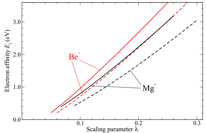
FIG. 1. Electron affinities of Be - and Mg - ions under the influence of the perturbation potential (11). Full lines are shown for the exponent \gamma = 0.025 , while the broken lines are for \gamma = 0.035 . Red color (light gray) describes the Be - ion and the black color is for the Mg - .
