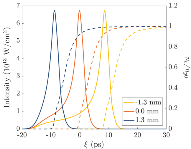
FIG. 6. The on-axis intensity of a flying pulse with v_f = -c at three axial locations. The persistence of a self-similar intensity profile, even with ionization dynamics, is evident.
