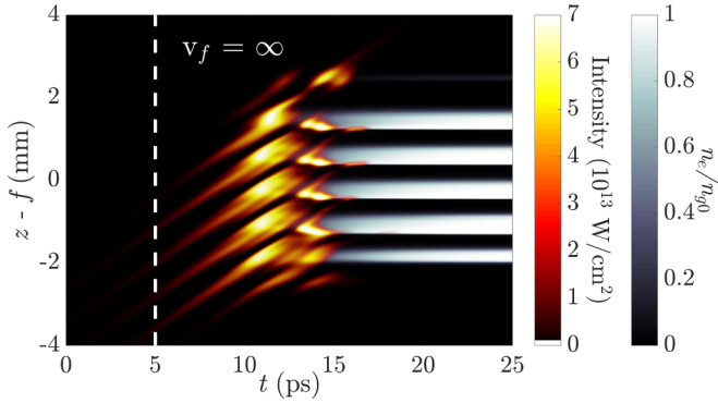
FIG. 8. Intensity and electron density as a function of axial location and time for a flying focus pulse with a modulated power spectrum and v_f = \infty , i.e., a simultaneous line focus. The diffractive lens has mapped the modulation in the power spectrum to a spatial intensity modulation. A modulated plasma density profile results.
