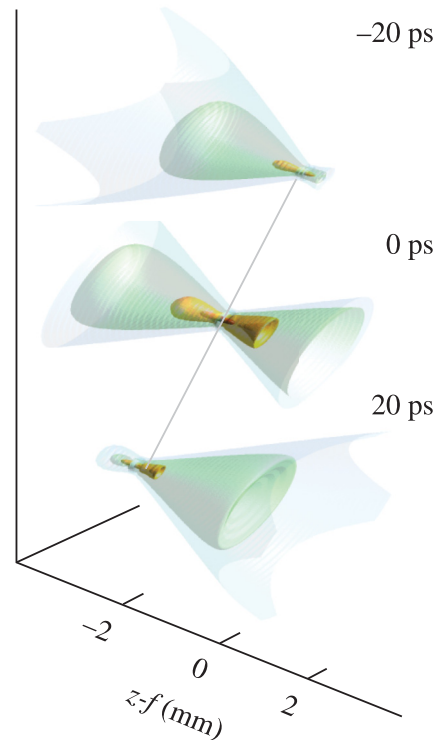
FIG. 3. Intensity isocontours of a flying focus pulse with v_f = -c/3 in the laboratory frame at three times, increasing from top to bottom. The peak intensity, represented by the dark orange contours, counterpropagates with respect to the optical axis.
