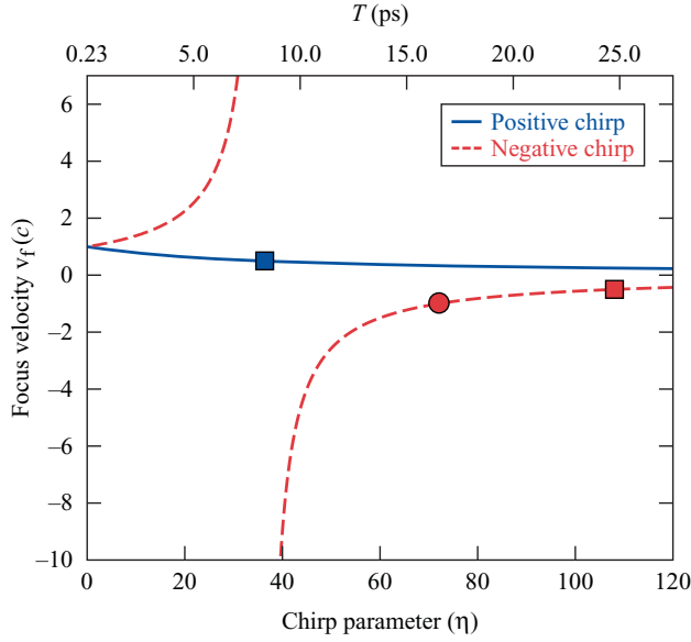
FIG. 2. The focal velocity of the flying focus pulse as a function of chirp parameter and pulse duration for the parameters in Table I. A positively chirped pulse is limited to positive focal velocities, while a negatively chirped pulse can have either a positive or negative velocity.
