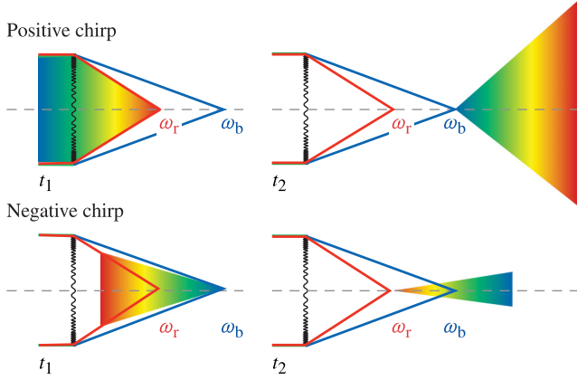
FIG. 1. Schematic of the flying focus. A positively (top row) or negatively (bottom row) chirped laser pulse passes through a diffractive lens. For the positive chirp, the red frequencies come to focus earlier than the blue, resulting in a positive focal velocity. For the depicted negative chirp, the blue frequencies come to focus earlier, resulting in a negative focal velocity.
