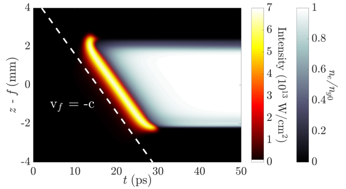
FIG. 4. Intensity and electron density as a function of axial location and time for a flying focus pulse with v_f = -c . The pulse creates a sharp ionization front that also travels at -c .
