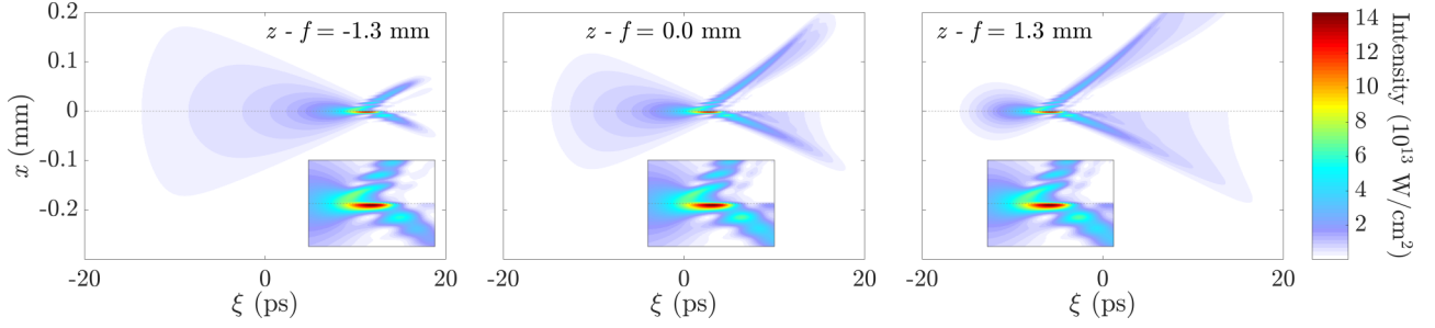
FIG. 5. Spatiotemporal intensity profiles of a flying pulse with v_f = -c at three axial locations. The profile in H_2 is plotted above the dashed line, and, to emphasize the effect of plasma refraction, the vacuum profiles are plotted below. The insets illustrate that, near peak intensity, a self-similar structure persists in both H_2 and vacuum as the flying focus traverses the focal region.
