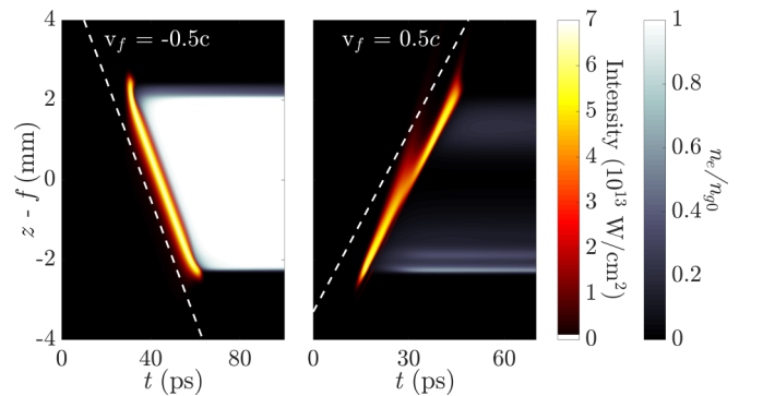
FIG. 7. Intensity and electron density as a function of axial location and time for flying focus pulses with v_f = -c/2 and v_f = c/2 on the left and right, respectively. The v_f = -c/2 pulse creates a sharp, clean ionization front, largely avoiding plasma refraction. The v_f = c/2 pulse suffers significant plasma refraction, producing an intermittent, disjointed ionization front.
