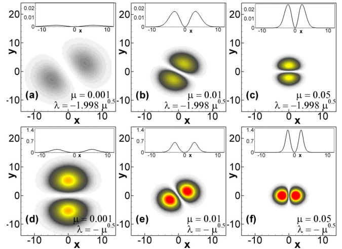
FIG. 5. Power plots and spatial profiles (top) of the dipole-mode multidimensional solitons for different parameters \mu and \lambda .
