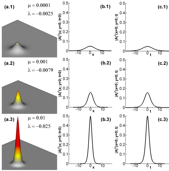
FIG. 3. Examples of three-dimensional solitons, shown for (a.1–a.3) power |A|^2(x,y,t) in the plane (x,y) for different \mu and \lambda = -0.25\sqrt{\mu} , and power profiles as cross sections in t and x .
