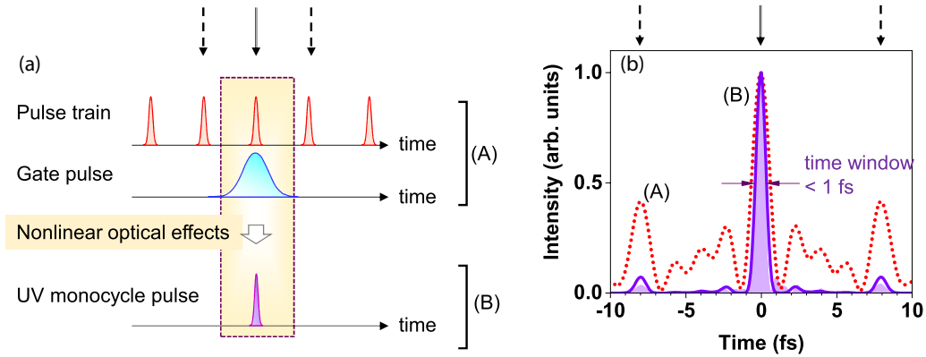
FIG. 1. (a) Schematic illustration of NOPS scheme. (b) Intensity of the incident synthesized pulse (dotted line, A), the attosecond time window (solid line, B), and the intensity of the UV radiation (solid area), which are the simulation results in Fig. 3(a) for the propagation length of 2 mm. Vertical arrows show the locations of the incident monocycle pulses.
