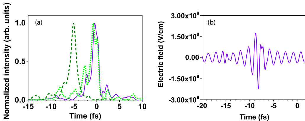
FIG. 4. (a) Normalized temporal intensity profiles of the UV radiations simulated for the gate-pulse intensities of 0.76 (broken line), 2.3 \times 10^{14} \text{ W/cm}^2 (dotted line), and 7.6 \times 10^{14} \text{ W/cm}^2 (solid line), respectively. (b) Simulated electric field of the UV radiation generated in the NOPS with the three incident spectral components.
