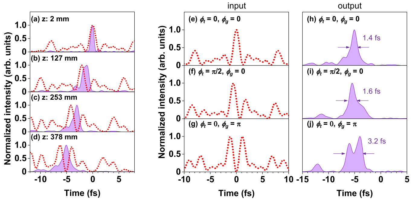
FIG. 3. (a)–(d) Simulated temporal intensities of the incident synthesized pulses (dotted line) and the UV radiation at propagation distances of (a) 2, (b) 127, (c) 253, and (d) 378 mm, respectively. Simulated temporal intensities of (e)–(g) the incident synthesized pulses at the entrance and (h)–(j) the UV radiations at the exit of the fiber (h)–(j). The CEPs of the incident radiations are (e), (h) \phi_t = \phi_g = 0 ; (f), (i) \phi_t = \pi/2, \phi_g = 0 ; (g), (j) \phi_t = 0, \phi_g = \pi .
