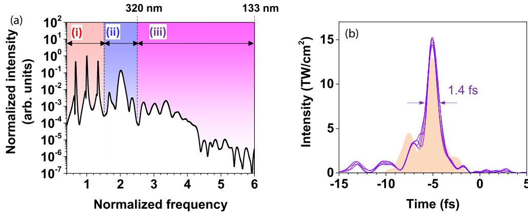
FIG. 2. Simulated (a) spectral and (b) temporal profiles. In (a), the frequency is normalized by that which corresponds to a wavelength of 800 nm. The spectral regions (i), (ii), and (iii), respectively, are of the incident pulse train, gate pulse, and the generated UV radiation. In (b), the temporal intensity profiles of the UV radiations simulated for the nine different phases are shown with solid lines. The solid area is the profile of the UV radiation generated by use of the pure isolated monocycle pulse and the gate pulse.
