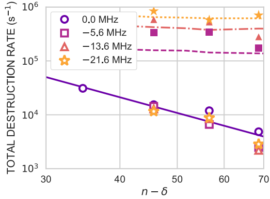
FIG. 7. Closed symbols: Rydberg molecule destruction rates, \Gamma_{\text{LOSS}} = (\Gamma_{\text{AI}} + \Gamma_L) , measured using the detunings, \gamma , indicated. The dashed, dot dashed, and dotted lines show the results of model simulations for detunings of -5.6 , -13.6 , and -21.6 MHz, respectively (see text). Open symbols: Decay rates, \Gamma_R , measured using thermal samples on atomic resonance [19] for zero detuning and L -changed atoms created in the BEC for finite detunings. The solid line indicates a fit to the decay rates measured on resonance.
