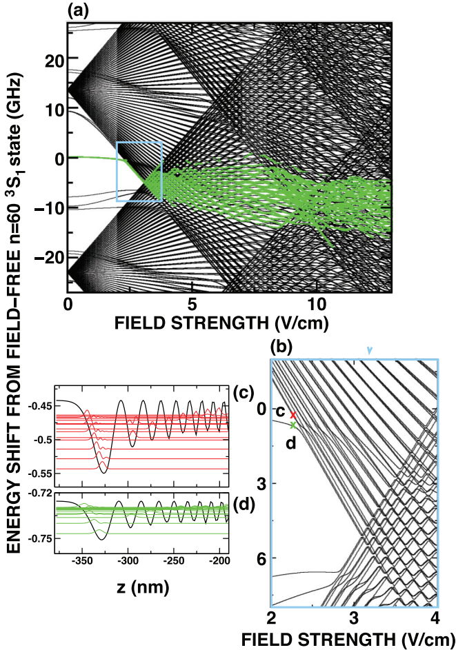
FIG. 3. (a) Calculated Stark energy level structure for M_J = 1 strontium atoms in the vicinity of the n = 60 ^3S_1 state. The green lines show the states with more than 1% occupation probability when ionizing the ^3S_1 state using a field with a slew rate of 43 \text{ V cm}^{-1} \mu\text{s}^{-1} . Panel (b) shows a portion of this structure on an expanded scale. Panels (c) and (d) show, respectively, the calculated molecular potentials, V(\vec{R}) , for a “dimer” molecule, formed from (c) the most red-shifted Stark state and (d) the parent n = 60 ^3S_1 state in a field of 2.3 \text{ V cm}^{-1} . The molecular wave functions, |\psi_\lambda(\vec{R}_g)|^2 , for the lowest-lying rovibronic levels ( \lambda = 1, 2, \dots, 16 ) are also shown (see text). Panels (c) and (d) show cross sections at \vec{R}_g = (0, 0, z) .
