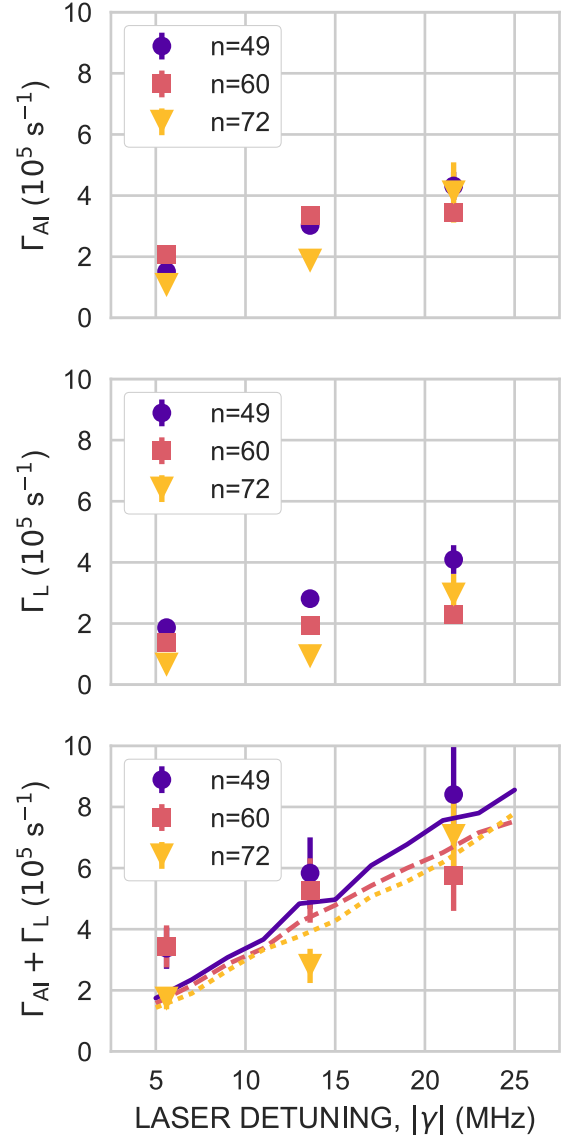
FIG. 8. Dependence of the reaction rates on detuning for the values of n indicated. Top: \Gamma_{\text{AI}} . Middle: \Gamma_L . Bottom: \Gamma_{\text{LOSS}} = (\Gamma_{\text{AI}} + \Gamma_L) . The results of model simulations are included using solid, dashed, and dotted lines for principal quantum numbers of 49, 60, and 72, respectively.
