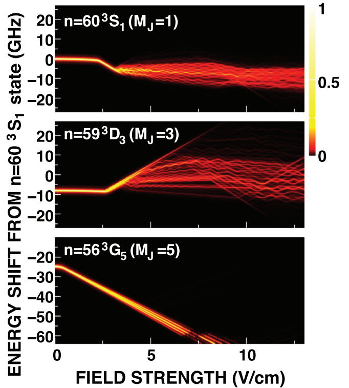
FIG. 4. Calculated time evolution of the occupation probability during ionization of the states indicated using a field with a slew rate of 43 \text{ V cm}^{-1} \mu\text{s}^{-1} . The calculated probability distribution is convoluted with a Lorentzian of 200 MHz in width.
