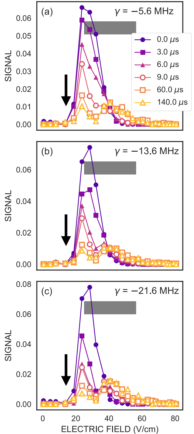
FIG. 5. Time evolution of the SFI signals recorded for n = 72 and the detunings, \gamma , indicated. The various time delays, t_D , are listed in the inset. The arrows and gray bars denote the threshold field for adiabatic ionization and the range of fields encompassed by purely diabatic ionization, respectively.
