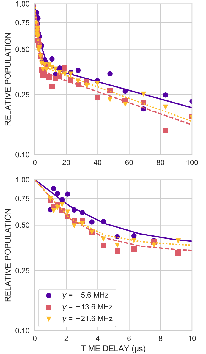
FIG. 6. Top: Time dependence of the total SFI signal for n = 49 and the detunings, \gamma , indicated. The data sets are each normalized to one at t = 0 . The solid, dashed, and dotted lines show fits to the data obtained using Eqs. (7) for detunings of -5.6 , -13.6 , and -21.6 MHz, respectively (see text). Bottom: Expanded view at early delay times.
