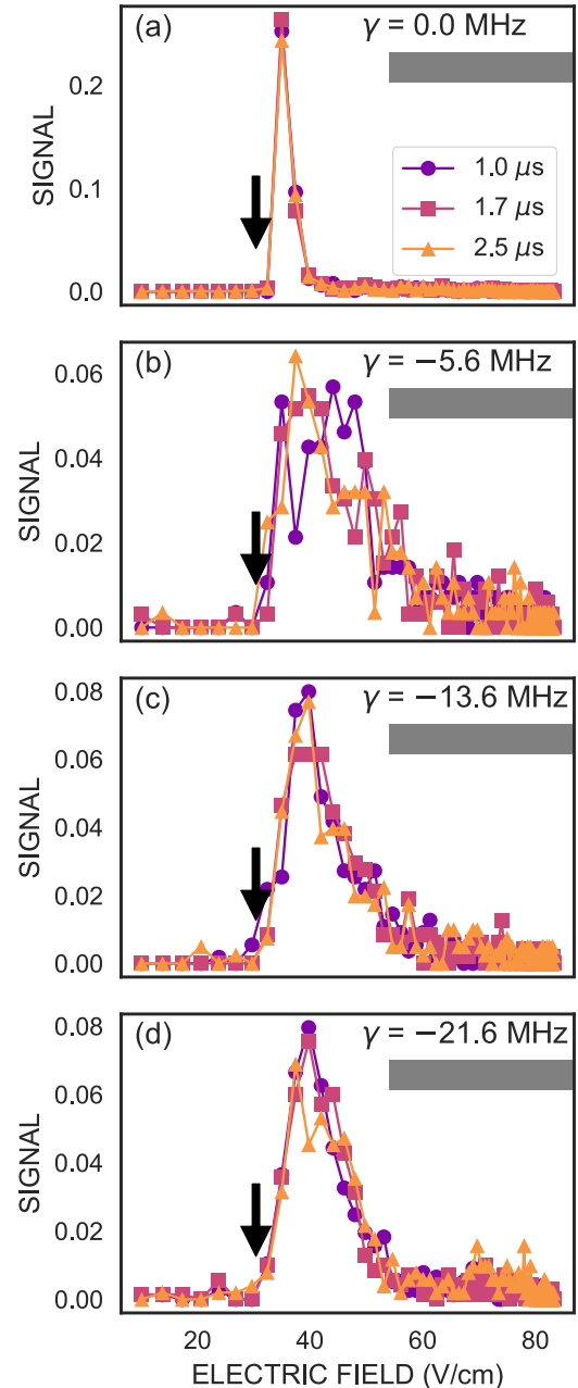
FIG. 2. SFI spectra recorded at n = 60 for the delay times t_D indicated. (a) Spectra obtained for the parent atomic state with the laser tuned to atomic resonance; (b)–(d) spectra recorded for Rydberg molecules with the detunings, \gamma , indicated. The arrows show the threshold field for adiabatic ionization [1/16(n - \delta)^4] ; the gray bars show the fields, which extend to \sim 120 \text{ V cm}^{-1} , over which purely diabatic ionization is expected. The various profiles in each figure are normalized to have equal areas.
