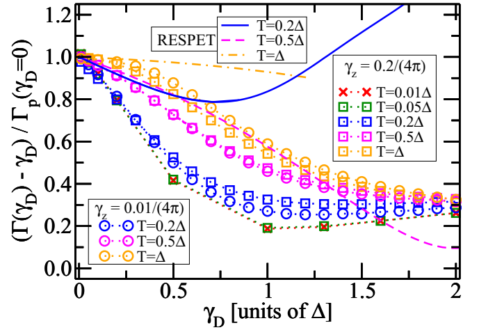
FIG. 2. The difference of decoherence rate and \gamma_D normalized by \Gamma_p(\gamma_D = 0) is plotted versus dephasing rate \gamma_D for five temperatures and two system-bath couplings and compared to the RESPET result [Eq. (7)].
