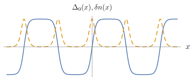
FIG. 1. Spatial variation in the FFLO state. Solid blue curve shows the order parameter or pair wave function \Delta_0(x) . Dashed yellow curve shows the density of unpaired fermions, \delta n(x) \equiv |n_\uparrow(x) - n_\downarrow(x)| . The unpaired fermions are localized near the domain walls.
