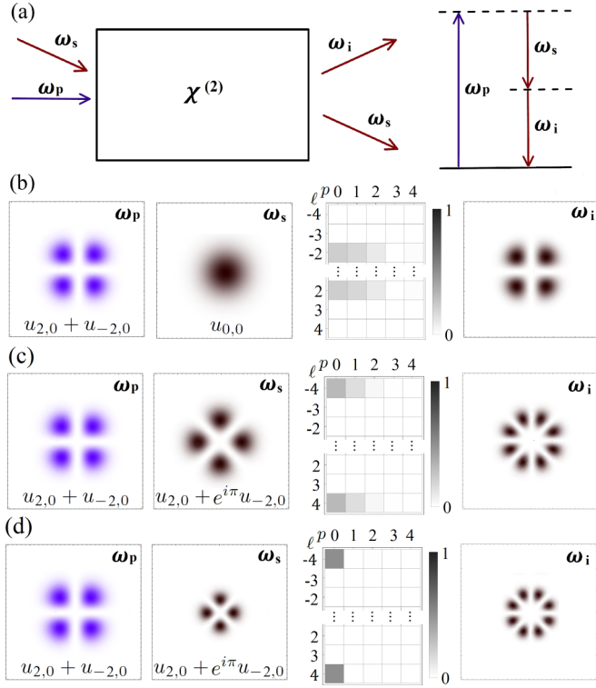
FIG. 2. In (a) we depict the simple stimulated-down-conversion scheme of our simulation. In (b) through (d) we show the input beam profiles of the pump and signal beams, a histogram giving the mode structure of the output (idler) beam, and the spatial profile of the output (idler) beam from left to right. In (b) we use a u_{0,0} signal as a baseline, and then in (c) and (d), we show how the signal beam can be chosen to tailor a clean higher OAM superposition in the idler mode.
