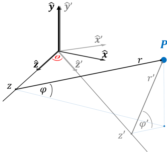
FIG. 7. Geometry of the two-beam coordinate systems, which are separated in the x - z plane by the angle \theta . Any point P can be described by the cylindrical coordinates (r, \phi, z) or (r', \phi', z') . We associate the generated beam with the unprimed coordinate system and the input beam with the primed coordinate system; then using geometry, we deduce the form of r', \phi', z' in terms of r, \phi, z , and \theta .
