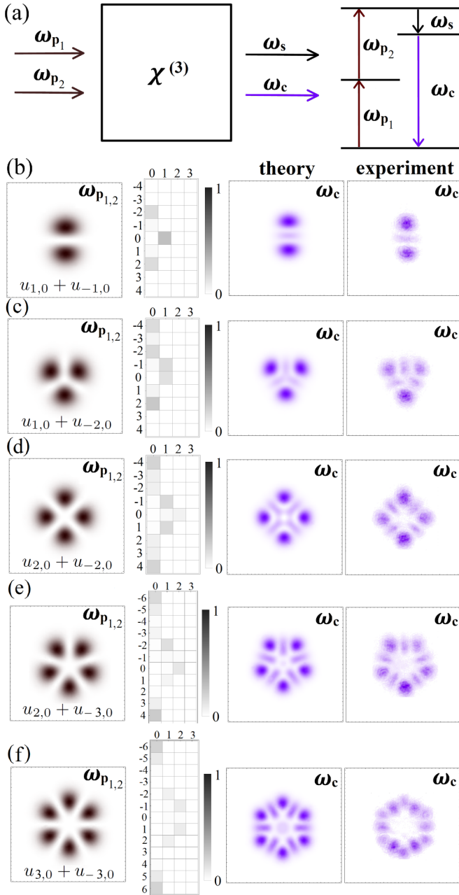
FIG. 3. In (a) we depict a nondegenerate four-wave mixing scheme, which occurs in ^{87}\text{Rb} . In (b) through (f), we study the result of this interaction for different pump profiles; from left to right the columns correspond to the profile of the pump beams, a histogram giving the mode structure of the conjugate beam, the spatial profile of the conjugate beam, and an experimental realization from Ref. [13]. Better qualitative agreement is observed when \omega_c is allowed to take on any mode conserving OAM. This result suggests that, contrary to previous assumptions, the long-wavelength signal beam can, in fact, carry OAM.
