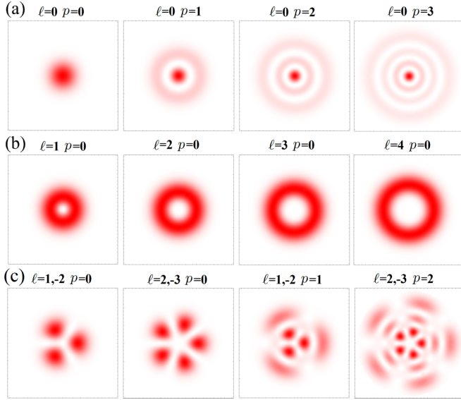
FIG. 1. LG mode intensity profiles for (a) \ell = 0 and increasing p , (b) p = 0 and increasing \ell , and (c) several superpositions of \ell with p = 0, 1 , and 2 . Due to interference, superpositions with \ell of opposite sign will have a symmetric petallike structure with |\ell_1| + |\ell_2| petals. See Ref. [2] for an excellent description of optical OAM origins and behavior.
