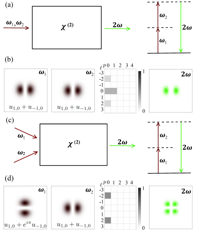
FIG. 4. In (a) and (c) we depict the two simple second-harmonic-generation schemes of our simulation. In (b) and (d) we show the input-beam profile, which is supplying the two pump photons; a histogram giving the mode structure of the output beam; and the spatial profile of the output beam from left to right. In (b) both pump photons come from a u_{1,0} + u_{-1,0} superposition. In (c) and (d), a phase shift and a new geometry are chosen such that destructive interference cancels the response at \ell = 0 [seen in (b)]. The pump photons are in the far infrared at 1140 nm, and thus, the second-harmonic response is at 570 nm.
