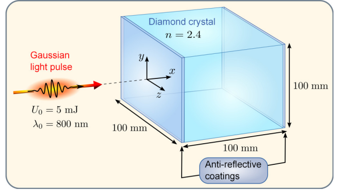
FIG. 4. The geometry of the simulations consisting of a cubic diamond crystal block coated with antireflective coatings. The refractive index of the crystal is n = 2.4 . A Gaussian light pulse of energy U_0 = 5 mJ and central wavelength \lambda_0 = 800 nm propagates in the direction of the positive x axis and enters the crystal from the left. The geometry is centered so that the center of the light pulse enters the crystal at x = y = z = 0 mm. The first interface of the crystal is located at x = 0 mm and the second interface at x = 100 mm.
