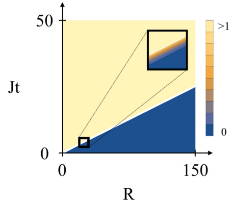
FIG. 1. Contour plot of I_R(4Jt) , the function controlling the bound on the fidelity of quantum state transfer in a spin chain [see Eqs. (5) and (26)]. The function is truncated above 1, the bound c \leq 2 always holds by the triangle inequality. A very sharp light cone with speed 6J emerges.
