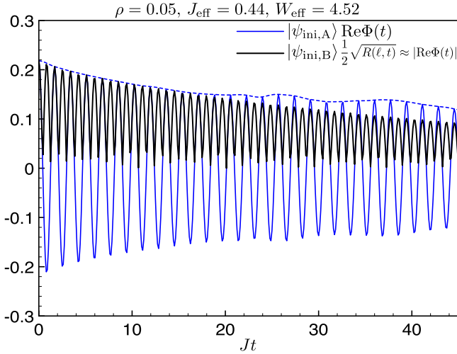
FIG. 12. Evolution of \text{Re}[\Phi(t)] for the initial state |\psi_{\text{ini},A}\rangle and system size L = 20 and |\text{Re}[\Phi(t)] calculated from \frac{1}{2}\sqrt{R(\ell,t)} for the initial state |\psi_{\text{ini},B}\rangle with separation \ell = 100 and system size L = 400 , both with density \rho = 0.05 . The dynamical Hamiltonian has J_{\text{eff}} = 0.44 and W_{\text{eff}} = 4.52 , chosen to reproduce the spin-flip quasiparticle dispersion and gap W_{\text{eff}} - 2J_{\text{eff}} = \Delta E = 3.64 in the original spin problem. The relaxation times obtained by fitting the exponential decay regime as in Figs. 9 and 11 are \tau_A \approx 46.5 and \tau_B \approx 51.0 respectively. This means that at time t = 18 —the longest time simulated in the original spin problem—the amplitude will be roughly 0.7 of the initial value.
