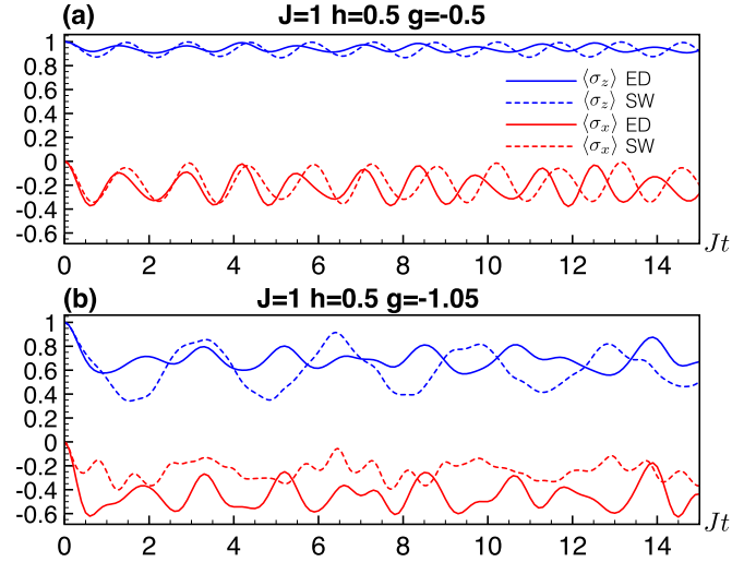
FIG. 5. Comparisons of the dynamics from ED and second-order SW for two different parameters for system size L = 13 . (a) g = -0.5 . The perturbative calculation is still quantitatively accurate at short time. The difference between ED and SW mostly comes from the difference between the exact and perturbative quasiparticle energy gap, resulting in the different oscillation frequencies. (b) g = -1.05 . The quantitative comparison becomes inaccurate at this parameter. For example, the oscillation frequency in the SW calculation is almost half of the ED calculation. Nevertheless, the SW calculation still captures the qualitative behavior observed in the ED calculation.
