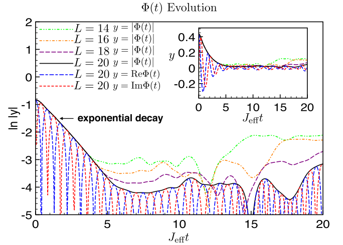
FIG. 6. ED results for \Phi(t) \equiv \langle b_j^\dagger(t) \rangle for the hard-core boson model, Eq. (10), and the product BEC state, Eq. (14), with average boson density \rho = |\beta|^2 = 0.25 , for system sizes L = 14, 16, 18, 20 . The parameters of the dynamical Hamiltonian are J_{\text{eff}} = 1 and W_{\text{eff}} = 5J_{\text{eff}} . Note that the main panel shows \ln |\Phi(t)| vs J_{\text{eff}} t , and the results strongly suggest exponential decay in t until recurrence time: as the system size increases, the time interval over which the exponential decay is observed also increases. Inset: linear scale for the observable. The recurrence times where the smaller-size results peel off from the largest-size results are roughly in agreement with those in Fig. 7.
