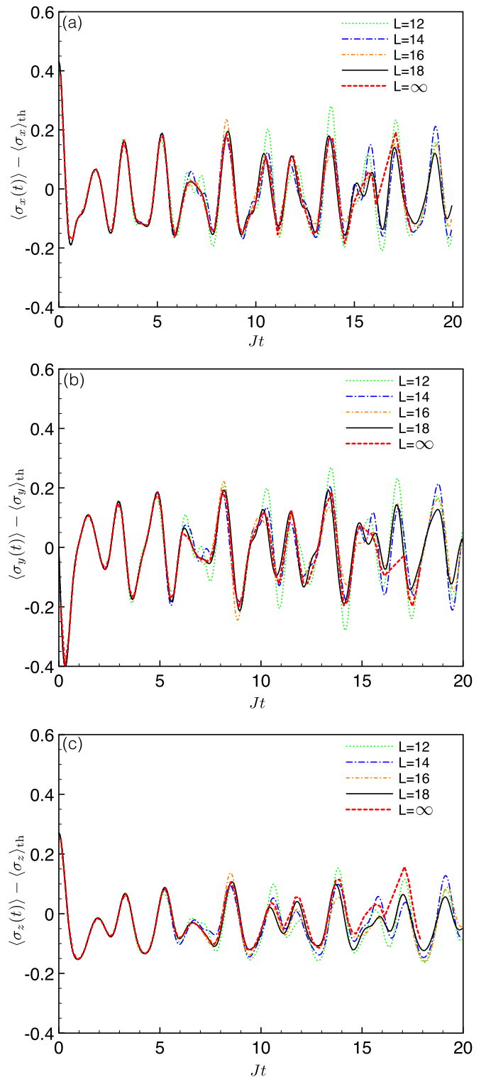
FIG. 1. (a)–(c) ED calculations of the evolution of some observables for several system sizes compared to infinite-MPS results from Ref. [37] marked as L = \infty (we are grateful to the authors of Ref. [37] for sharing their data with us). For smaller L , visible deviations from the L = \infty results appear at smaller t , which we associate with recurrence phenomenon in finite systems. Close agreement of our ED results with the infinite-MPS results over a large time window allows us to identify the frequency of the oscillations from finite-size spectra, which we argue is essentially the quasiparticle energy at zero momentum.
