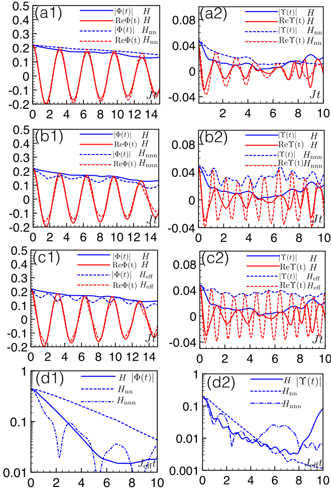
FIG. 13. Comparison of the dynamics under the simplified hard-core boson Hamiltonian H in Eq. (10) and under various Hamiltonians with different additional interactions. The initial state is |\psi_{\text{ini},A}\rangle . (a)–(c) BEC order parameter (left panels) and pair boson correlation function (right panels) for density \rho = 0.05 and system size L = 14 . The parameters of H_{\text{eff}} are obtained from second-order SW for the original spin model, and similar parameters are also used in H , H_{\text{nn}} , H_{\text{nnn}} : J_{\text{eff}} = 0.88 , W_{\text{eff}} = 3.68 , W_{\text{nn}} = -0.47 , and W_{\text{nnn}} = 2.35 (in units of J ). The additional interactions basically introduce a small amplitude oscillation in \Phi(t) . For the pair-boson correlation function, the decay behavior and the oscillation frequencies are affected more strongly (see text for details). (d) BEC order parameter \Phi(t) and pair-boson correlation function \Upsilon(t) for density \rho = 0.25 , system size L = 20 and parameters J_{\text{eff}} = 1.0 , W_{\text{eff}} = 1.0 , W_{\text{nn}} = -0.5 , and W_{\text{nnn}} = 1.5 (the results for H are identical as in Figs. 6 and 7). The additional interaction of the JW fermions in H_{\text{nn}} changes the decay in \Upsilon(t) to be faster than the previous power law.
