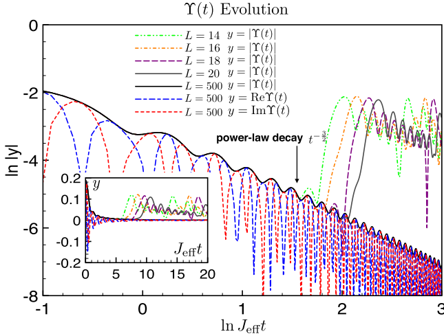
FIG. 7. ED results for \Upsilon(t) \equiv \langle b_j^\dagger(t)b_{j+1}^\dagger(t) \rangle for the same systems as in Fig. 6 with average density \rho = 0.25 . This observable can be also calculated analytically using Jordan-Wigner transformation (checked against ED for small L ), allowing us to study much larger sizes and times, as illustrated here for L = 500 . Note that the main panel shows log-log plot, and the long-time behavior in the largest system clearly has a power-law envelope with decay t^{-3/2} , in agreement with the analytical calculation in the text. Inset: linear scale for the observable. By comparing data for L = 14, \dots, 20 and much larger L = 500 , we can also clearly see where the recurrences appear for the smaller sizes.
