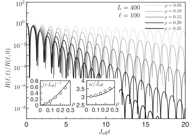
FIG. 11. R(\ell, t) as in Fig. 10 but for different average densities \rho obtained by tuning \mu_0 and \Delta_0 according to Eqs. (35) and (36) respectively. We show only the largest separation \ell = 100 ; the full system size is L = 400 and is sufficiently large to reflect the thermodynamic limit in L . The values are normalized by the initial value in order to bring out the decay rate, which clearly increases as the density increases. Insets: inverse relaxation time \tau^{-1} of the exponential decay and the oscillation frequency \omega as a function of density, obtained from fitting the data in the main panel to form Ae^{-2t/\tau} \cos^2(\omega t - \alpha) + C . The circle symbols denote the fitted values, while the solid lines denote the conjectured forms Eqs. (23) and (24) for \tau^{-1} and \omega respectively (see text for details).
