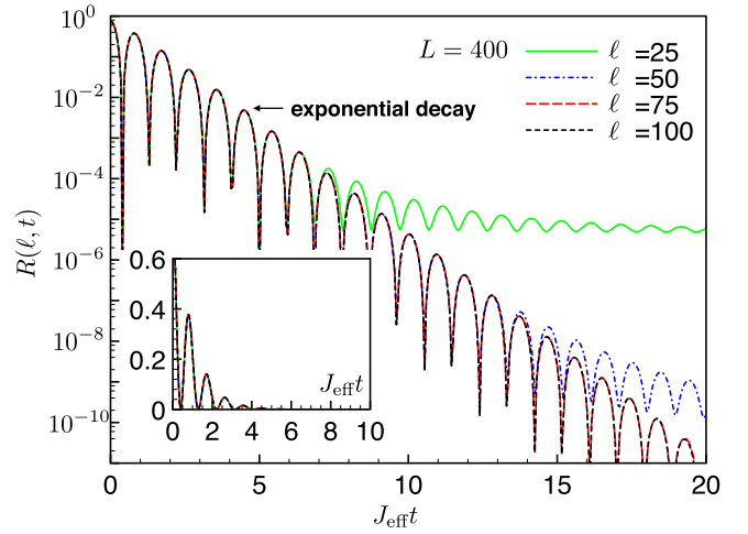
FIG. 10. Numerical results for R(\ell, t) obtained using the Pfaffian method; the system size is L = 400 , and we consider separations \ell = 25, 50, 75 , and 100 . The initial state is the ground state of Eq. (25) with parameters \Delta_0 = 0.60 and \mu_0 = -1.60 , corresponding to particle density \rho = 0.25 . The parameters of the dynamical Hamiltonian are chosen as J_{\text{eff}} = 1 and W_{\text{eff}} = 5 . We are primarily interested in the regime t \ll \ell/v , where v is some information-spreading velocity. In this regime, the observable exhibits exponential decay. The time interval over which we see the exponential decay increases as the separation \ell increases.
