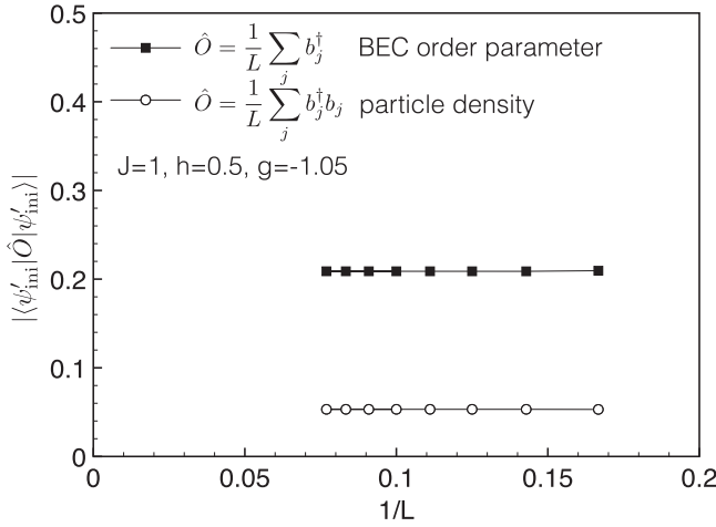
FIG. 4. Properties of the SW-rotated initial state |\psi'_{\text{ini}}\rangle = e^{iS}|\psi_{\text{ini}}\rangle , with iS = iS^{[1]} + iS^{[2]} calculated to second order in g (see Appendix A for details). The figure shows expectation values of the particle density b_j^\dagger b_j \equiv (1 - \sigma_j^z)/2 and BEC order parameter b_j^\dagger \equiv (\sigma_j^x - i\sigma_j^y)/2 . The particle density \rho \approx 0.05 is very low and close to the estimate based on the average energy density in the initial state and the quasiparticle gap.
