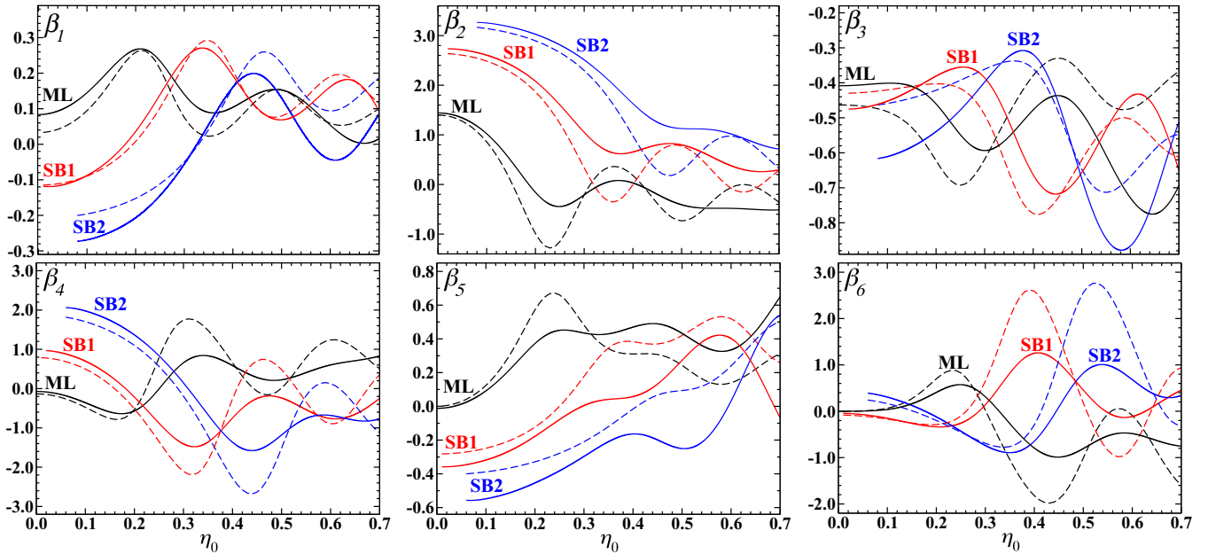
FIG. 5. Anisotropy parameters \beta_k ( 1 \leq k \leq 6 ), for \varphi_X = 0 , as a function of the IR-field amplitude ratio \eta_0 . Labels are the same as in Fig. 4.
