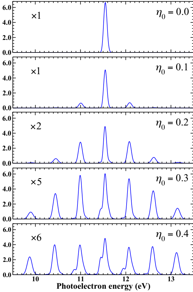
FIG. 3. TDSE results for the ionization probability (in units of 10^{-3} \text{ eV}^{-1} ) as a function of the photoelectron energy for different IR-field amplitude ratios \eta_0 . The fundamental XUV intensity is I = 10^{12} \text{ W/cm}^2 , \eta_X = 0.1 , and the infrared frequency is \Omega_0 = 0.55 \text{ eV} .
