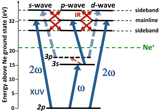
FIG. 1. Scheme of the \omega + 2\omega + \Omega_0 process in neon in the dipole approximation. The ionization is caused by the fundamental and second harmonics (solid blue arrows) of an XUV pulse whose fundamental frequency \omega is tuned near the 2p \rightarrow 3s transition. The overlapping IR field induces ATI (small red arrows) transitions leading to sidebands in the spectrum. Only s , p , and d waves are displayed, although higher partial waves can contribute. Dashed arrows represent additional paths created when the IR frequency is tuned near the 3s \rightarrow 3p transition (see text).
