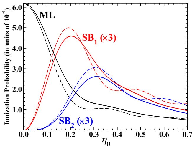
FIG. 4. Ionization probability associated with the different bands calculated in the TDSE (solid lines) and the SFA (dashed lines) approaches as a function of the IR-field amplitude ratio \eta_0 .
