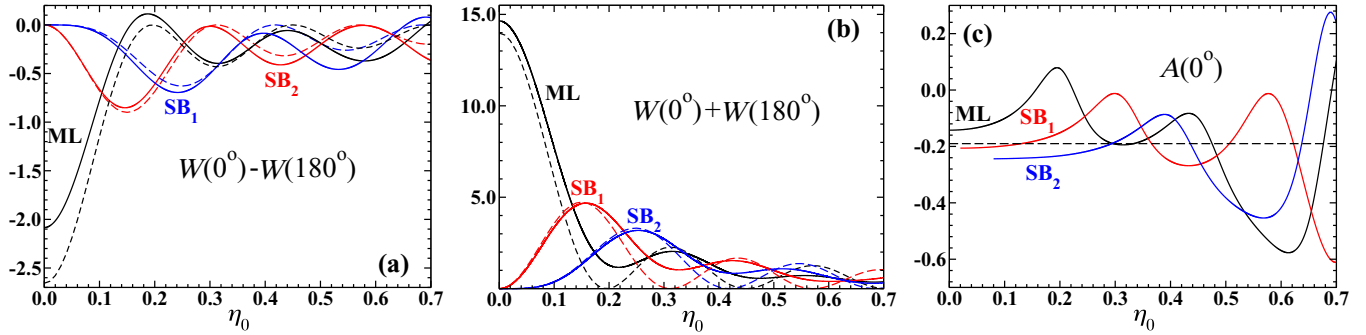
FIG. 6. (a) Subtracted and (b) summed forward and backward ionization probability signals (in units of 10^{-4} ), as well as (c) left-right asymmetry, as a function of the IR-field amplitude ratio \eta_0 , as calculated in the TDSE and SFA approaches. Note the constant value of A(0^\circ) in the SFA.
