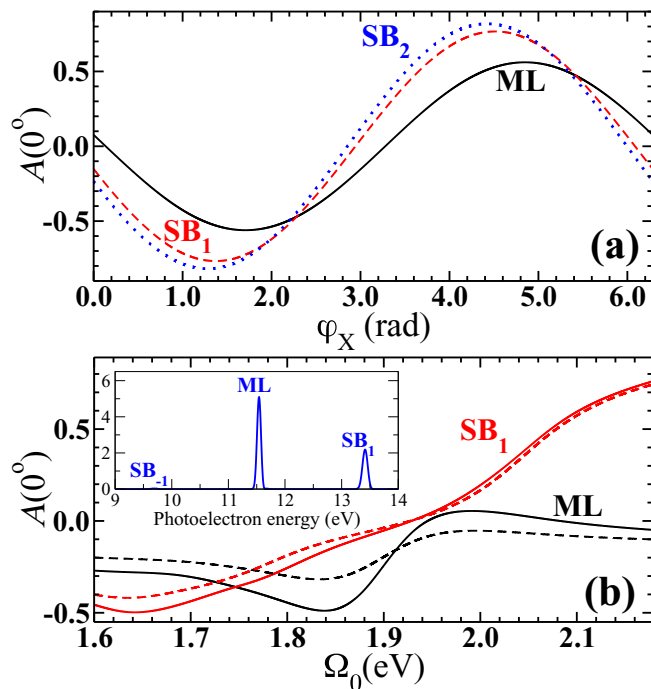
FIG. 7. (a) Left-right asymmetry A(0^\circ) for ML (solid black line), SB 1 (dashed red line), and SB 2 (dotted blue line), as a function of \varphi_X at \Omega_0 = 0.55 eV and \eta_0 = 0.2 . (b) Left-right asymmetry A(0^\circ) as a function of the IR frequency \Omega_0 at \eta_0 = 0.2 (dashed lines) and \eta_0 = 0.3 (solid lines). Inset: Corresponding ionization probability spectrum (in units of 10^{-3} eV ^{-1} ) at \eta_0 = 0.3 .
