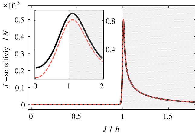
FIG. 3. Solid black line: Specific QFI for the estimation of J in the XX model versus J/h . As in Fig. 1 the ferromagnetic phase has been shaded. Dashed red line: Specific J sensitivity F(J; \hat{J}_z)/N of the total magnetization \hat{J}_z . The temperature was set to \beta = 100 , h = 1 , and N = 10^3 . Inset: Same as in the main plot for the much larger temperature \beta = 2 . Note that, unlike in the main plot, the vertical axis of the inset is not scaled by the 10^3 factor.
