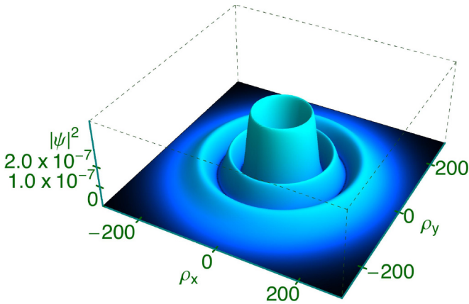
FIG. 2. Plot of the probability density |\psi(\vec{\rho})|^2 for a bound electron in a state with quantum numbers n = 12, \ell = 9 , and m = 9 , in the field of the same charged black hole as given in Fig. 1. The quantum numbers are n = 12, \ell = 9 , and m = |\ell| = 9 , and the polar angle is \theta = 90^\circ , i.e., the plot pertains to the (\rho_x, \rho_y) plane, with the dimensionless vector-valued variable \vec{\rho} being defined in Eq. (30).
