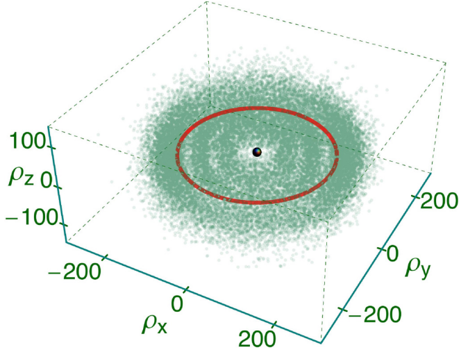
FIG. 1. Scatter plot of the probability density of finding a bound particle (electron) in a state of n = 12, \ell = 9 , and m = |\ell| = 9 in the field of a charged heavy black hole with mass 10^{-12} times the mass of the earth, and charge number Z_Q = 10 . The points are distributed randomly, with the number of scattered points in a reference volume being proportional to the probability of finding the bound electron in the volume. The two radial minima of the probability density are clearly visible. The gravitational center is depicted as a black dot. For reference, the classical trajectory at \langle \rho \rangle = \int \rho |\psi(\vec{\rho})|^2 d^3r = 171 is also shown. Note that the scaled radial coordinate \vec{\rho} given in Eq. (30) is dimensionless, as reflected in the labeling of the axes.
