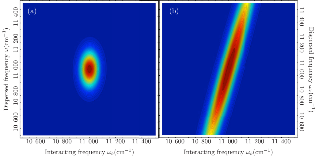
FIG. 5. (a) Absolute value of the product of uncorrelated classical light envelopes, E_{pr}^*(\omega)E_{pr}(\omega_b) , with \sigma = 100 \text{ cm}^{-1} . (b) Absolute value of the coherent correlation function, Eq. (B5), of degenerate, entangled photon pairs with \sigma_p = 400 \text{ cm}^{-1} , T = 900 \text{ fs} .
