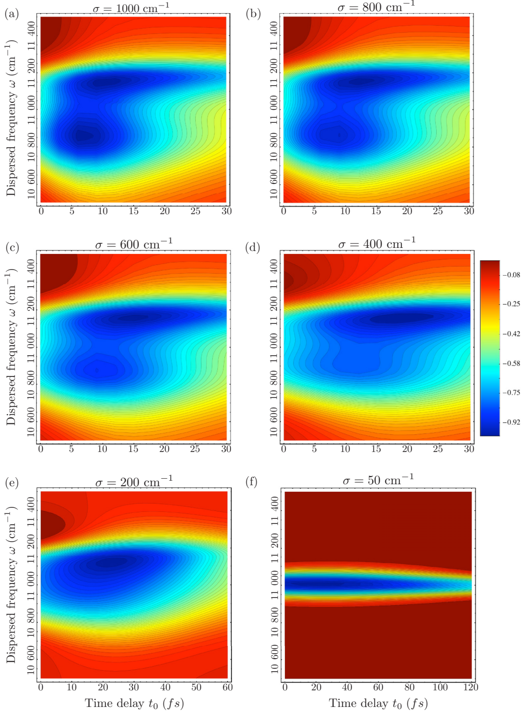
FIG. 2. The classical pump-probe signal, Eq. (16), displayed vs the time delay to the pump pulse t_0 (in fs), and the dispersed frequency \omega (in \text{cm}^{-1} ) with a probe bandwidth of (a) \sigma = 1\,000 \text{ cm}^{-1} (i.e., 5.6 fs), (b) 800 \text{ cm}^{-1} , (c) 600 \text{ cm}^{-1} , (d) 400 \text{ cm}^{-1} , (e) 200 \text{ cm}^{-1} , and (f) 50 \text{ cm}^{-1} (111 fs). The center frequency of the probe beam is fixed at \omega_0 = 11\,000 \text{ cm}^{-1} .
