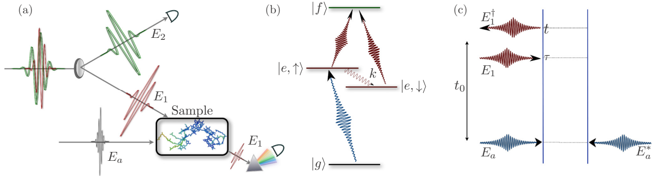
FIG. 1. (a) The proposed TPC setup: the entangled photon pair in beams E_1 and E_2 are split on a beam splitter. A classical, actinic, ultrafast pulse E_a excites the sample, and E_1 is employed as a probe in a pump-probe measurement, while E_2 is spectrally dispersed, and detected in coincidence. (b) The level scheme for the two-state jump (TSJ) model considered in this work. The g - e transition is driven by the actinic pulse (blue arrow). It is far off-resonant from the spectral range of the entangled photon wave packet (red arrows), which only couples to the e - f transition. (c) Ladder diagram representing the pump-probe measurement.
