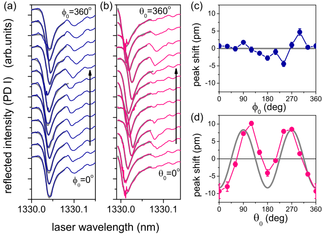
FIG. 3. (Color online) Reflected intensity (PD I) on a single resonance as a function of (a) in-plane angle \phi_0 ( \theta_0 = 90^\circ ) and (b) out-of-plane angle \theta_0 ( \phi_0 = 45^\circ ) of the magnetization with respect to the WGM plane. The fitted gray lines are used to extract (c), (d) the resonant frequency as a function of the two angles. The gray lines in (c) and (d) are the expected shifts considering only the Voigt effect given by Eq. (9).
