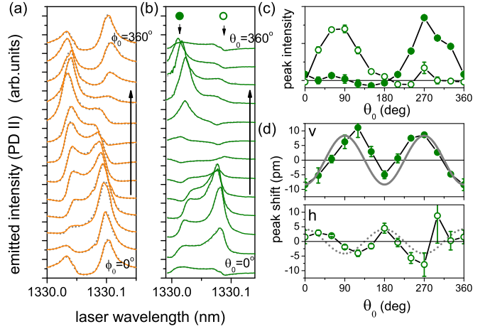
FIG. 4. (Color online) Emitted intensity from WGM with horizontal linear polarization (PD II), opposite to the input beam. Emitted intensity as a function of laser wavelength for (a) in-plane angle \phi_0 and (b) out-of-plane angle \theta_0 of the magnetization. Gray dotted lines are double peak fit to data. (c) Peak intensity of the two peaks as a function of out-of-plane angle \theta_0 [from fitting in (b)]. (d) Wavelength shift of the two peaks as a function of out-of-plane angle \theta_0 . The gray lines are the expected dependence based on Voigt effect, same as Fig. 3, for the two modes with mainly vertical (solid) and horizontal (dotted) linear polarizations.
