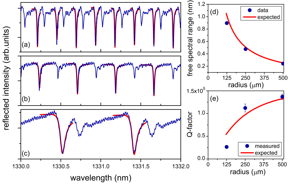
FIG. 2. (Color online) Reflected intensity (PD I) as a function of input laser free-space wavelength \lambda for varying radius YIG spheres: (a) 500 \mu\text{m} , (b) 250 \mu\text{m} , and (c) 125 \mu\text{m} . Red lines are separate fits to each peak, which give (d) the peak separation (free spectral range) and (e) Q factors. The red line in (d) is the expected free spectral range for the WGMs, \Delta\lambda , given by Eq. (1), and the red line in (e) is the expected Q factor.
