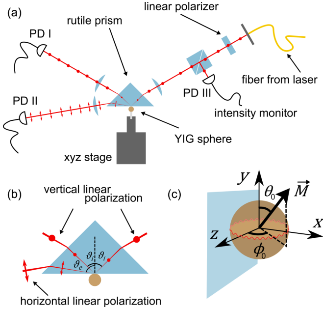
FIG. 1. (Color online) (a) Schematic of experimental setup. The light from the fiber-coupled laser is collimated, linearly polarized vertically (perpendicular to the plane), and focused onto the internal surface of the coupling prism. Two photodiodes on the output of the prism monitor the reflection of the input beam with vertical polarization (I) and the emission of any horizontally linear polarized light (II) from the YIG sphere. To account for fluctuations in laser intensity, all measurements are normalized to the input power monitored with a beam splitter and photodiode (III) on the input path. The YIG sphere is mounted on a xyz positioning stage to locate it at the coupling point. (b) The optical axis of the birefringent rutile prism is out-of-plane, which separates the output angles of the two linear polarizations for analysis via the two photodiodes. (c) Definition of the polar ( \phi_0 ) and azimuthal ( \theta_0 ) angles of the magnetization \vec{M} .
