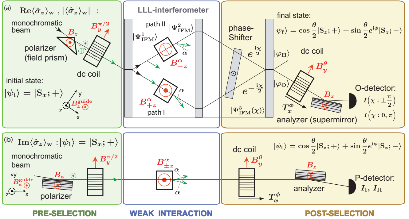
FIG. 1. (Color online) Schematic illustration of experimental apparatus for full determination of the weak value of the Pauli spin operator \hat{\sigma}_z of system S . (a) Triple Laue (LLL) neutron interferometer (IFM) setup for determination of the real component and modulus of \langle \hat{\sigma}_z \rangle_w . (b) Polarimetric setup for the imaginary part of \langle \hat{\sigma}_z \rangle_w , where no interference effects are necessary. The procedure consists of three stages: (i) preselection (green); using a polarizer (initial polarization is along +z direction) and a \pi/2 spin rotator the initial state |\psi_i\rangle = |S_x; +\rangle is prepared. (ii) Weak interaction (blue); in case (a) after the beam splitting a weak spin rotation by \pm\alpha is applied in arms I and II. In case (b) a spin rotation by \pm\alpha is applied directly after the preparation of the initial state |\psi_i\rangle . (iii) Postselection (yellow); a combination of a spin rotator and an analyzing supermirror is used to postselect the final spin state |\psi_f(\theta, \phi)\rangle = \cos(\frac{\theta}{2})|S_z; +\rangle + \sin(\frac{\theta}{2})e^{i\phi}|S_z; -\rangle , followed by a count rate detection. In case (a) the pointer readout, i.e., tuning of the path state |\varphi_0\rangle , being the two-level probe system P , is achieved by a rotating phase-shifter plate, inducing a relative phase \chi between the path eigenstates |I\rangle and |II\rangle .
