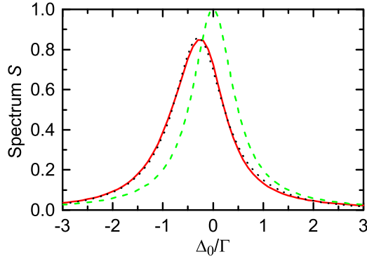
FIG. 5. (Color online) Expected spectral line shapes. The red solid line shows the expected line shape numerically calculated from Eq. (A11) for the typical values for our experiment from Eq. (A13). This line is broadened and shifted because of the nonzero width of the thermal atomic position distribution. The black dotted line is a Lorentzian fit to this. The green dashed line shows the Lorentzian reference for \tau_1 = \tau_2 = 0 , corresponding to a classical particle located exactly at the trap center.
