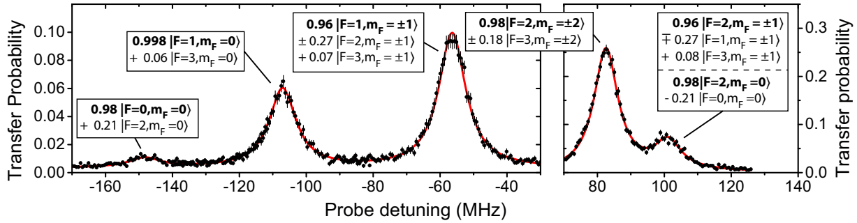
FIG. 3. (Color online) Measured excitation spectrum of a single ^{87}\text{Rb} atom for transitions from the 5S_{1/2}, F = 1 ground state to 5P_{3/2} excited states. A probe light pulse transfers populations into the F = 2 ground state by optical pumping, whenever resonant with an atomic transition. The final populations are measured. Five atomic resonance lines are clearly resolved. The line shows a fit of the sum of five Lorentzians with independent amplitudes, widths, and center frequencies. The boxes label energy eigenstates that we assign to the 5P_{3/2} excited states causing these resonances, where terms with amplitudes below 0.01 are omitted. Without hyperfine breakdown, this frequency range would show only three lines, because the two rightmost lines would be degenerate and the leftmost line would be a forbidden transition.
