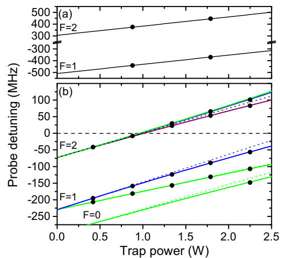
FIG. 4. (Color online) Quantitative analysis of differential light shifts. Solid lines show fits to the experimentally observed line centers (dots). Dotted lines show linear approximations for low power. The data cover the (a) 5S_{1/2} \leftrightarrow 5P_{1/2} and (b) 5S_{1/2} \leftrightarrow 5P_{3/2} transitions in ^{87}\text{Rb} . Note that unlike Fig. 1, these data show differential light shifts.
