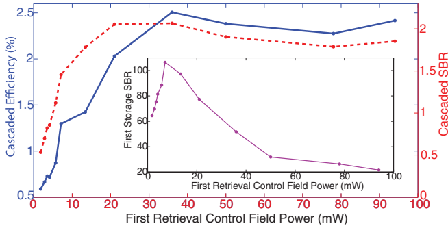
FIG. 5. (Color online) Total cascaded storage efficiency \eta_T (gray line [blue online]) and cascaded SBR (dashed gray line [red online]) vs optical power for first retrieval. Inset: SBR of first storage event vs optical power for first retrieval (purple online).
