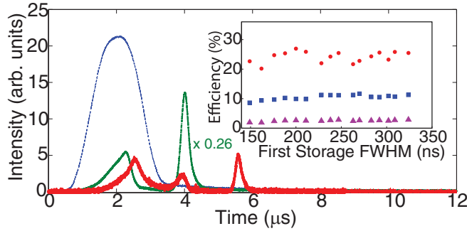
FIG. 3. (Color online) Successive storage of classical pulses. Thin gray line [blue online]: input pulse; gray line [green online]: rail 1 single storage signal; thick gray line [red online]: rail 2 cascaded storage signal. The gray line [green online] is scaled by a factor 0.26 to account for different propagation losses after the first and second rails. Inset: dependency of storage efficiencies on the full-width half maximum of the Gaussian shaped retrieved field for the first storage. Squares [blue online]: efficiency of the first storage \eta_1 ; circles [red online]: efficiency of the second storage \eta_2 ; and triangles [purple online]: overall efficiency of cascaded storage procedures \eta_T .
