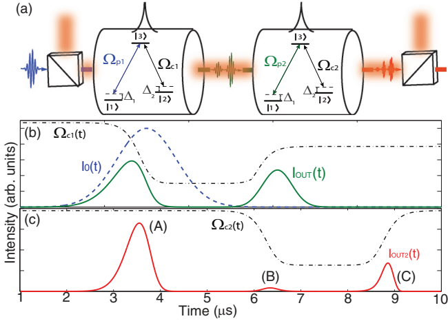
FIG. 1. (Color online) (a) Concept of the cascaded storage with two light-matter interfaces. (b) First storage: Input pulse (dashed line [blue online]), control field 1 time sequence (dot-dashed line [black online]), and retrieved light signal (solid line [green online]) as obtained by simulation. (c) Second storage: control field 2 time sequence (dot-dashed line [black online]), notice the time delay with respect to control field 1 and cascaded retrieved signal (solid line [red online]).
