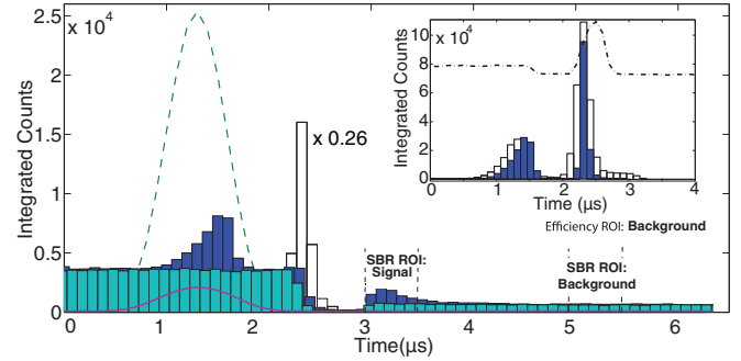
FIG. 4. (Color online) Cascaded optical storage for input pulses containing eight photons per pulse on average. Dashed line [green online]: input pulse (measured in SPCM 2); light gray line [purple online]: absorbed pulse (measured in SPCM 2); white bars histogram: retrieved pulse after first storage (measured in SPCM 1 scaled by a factor 0.26); gray bars histogram [blue online]: retrieved signal after cascaded storage procedure (with background, measured in SPCM 2); light gray bars histogram [blue online]: background-only measurement. Inset: The effect of reshaping the control field for the optical retrieval in the first rail. Storage using on-off modulation of control field 1 (grey bars histogram [blue online]) and storage counts obtained with a temporally modulated control field 1 (white bars histogram). The temporal shape of the control field 1 is indicated by the dotted black line.
