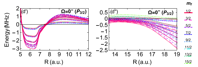
FIG. 12. (Color online) Zooms of the ^{40}\text{KCs} 0^-(P_{3/2}) DPECs of Fig. 8(d) for ranges of R in between the peaks marking the transition from one Hund's case a character to the other.
