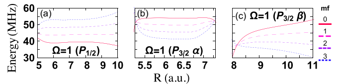
FIG. 13. (Color online) Zooms on the R intervals for which the ^{39}\text{KCs} 1(P_j) DPECs of Fig. 5 are grouped according to the projection of the nuclear spin of the cesium and potassium atoms. The figure displays the four curves m_{i_{^{39}\text{K}}} = -3/2, \dots, 3/2 associated with the fourth pack (counting from the top) in the case of the ^{39}\text{K}^{133}\text{Cs} molecule.
