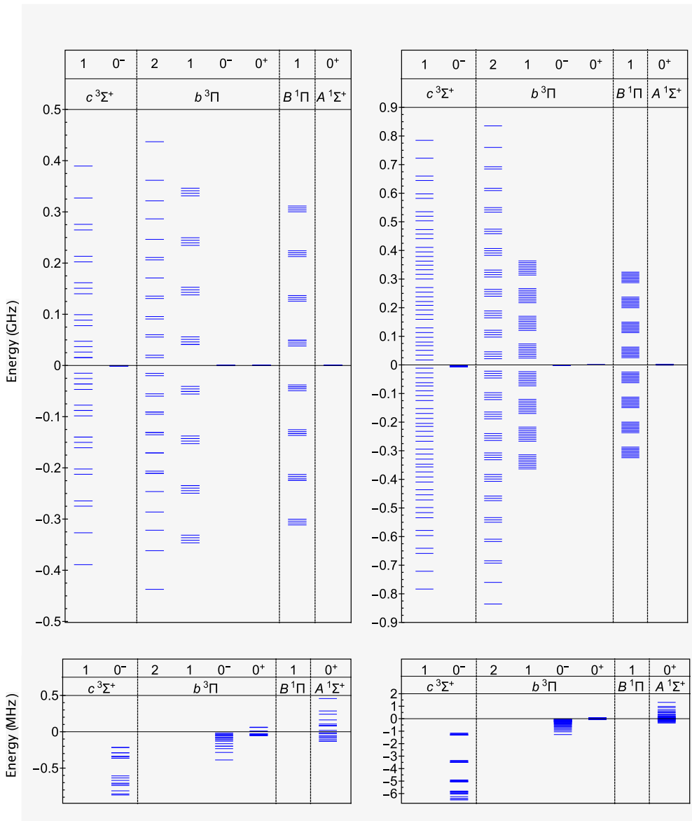
FIG. 15. (Color online) Difference potential energies of the Hund's case c states at R = 10.5 a.u. of (left) the bosonic ^{39}\text{KCs} and (right) fermionic ^{40}\text{KCs} molecules. The bottom panels display zooms for the \Omega = 0 states. Both the relevant Hund's case c states and the dominant Hund's case a character are indicated. For Hund's case c notation in the upper line we have used a simplified one giving only the value of \Omega . From column 1 to column 8 the order of the states is 1(P_{3/2} \alpha) , 0^-(P_{3/2}) , 2(P_{3/2}) , 1(P_{1/2}) , 0^-(P_{1/2}) , 0^+(P_{1/2}) , 1(P_{3/2} \beta) , and 0^+(P_{3/2}) .
