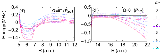
FIG. 10. (Color online) Zooms of the ^{39}\text{KCs} 0^-(P_{3/2}) DPECs of Fig. 7(d) for ranges of R in between the peaks marking the transition from one Hund's case a character to the other.
