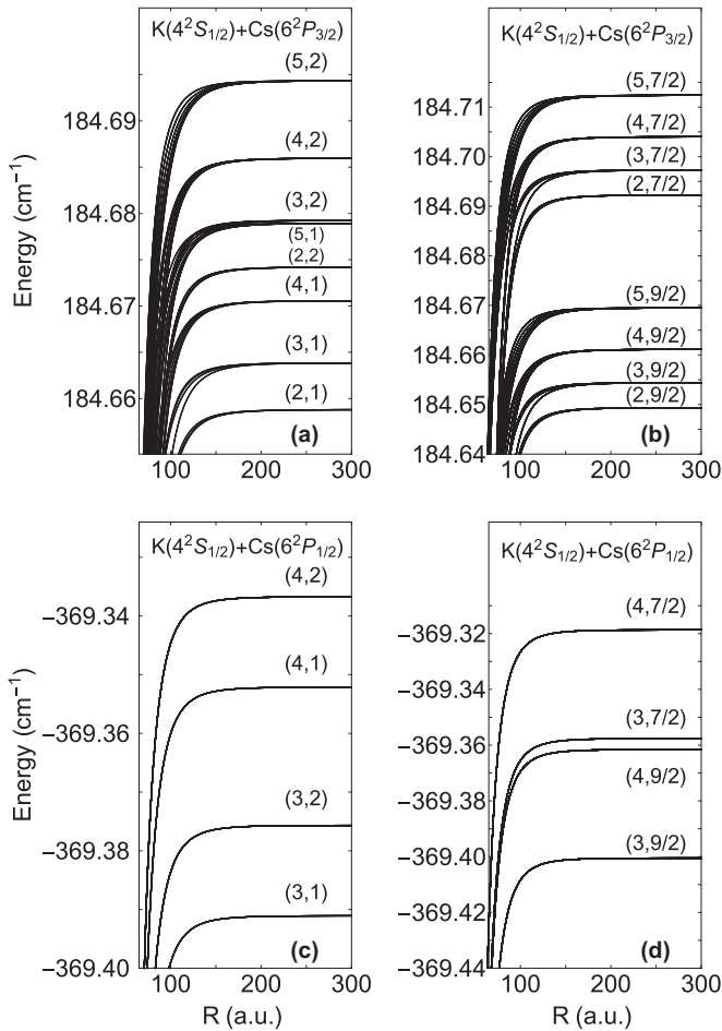
FIG. 4. Long-range potential-energy curves (PECs) of KCs including hyperfine interaction, correlated to \text{K}(4^2S_{1/2}, f_1) + \text{Cs}(6^2P_{j_2}, f_2) . (a) and (c) The 216 PECs of ^{39}\text{KCs} . (b) and (d) The 432 PECs of ^{40}\text{KCs} . Hyperfine dissociation limits are labeled with (f_1, f_2) .
