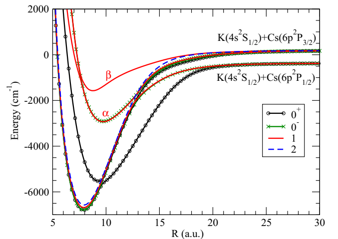
FIG. 2. (Color online) Hund's case c potential-energy curves of excited molecular states correlating to the dissociation limits K(4^2S_{1/2}) + Cs(6^2P_{1/2,3/2}) . The \alpha and \beta indexes label the two \Omega = 1 states correlated to the upper dissociation limit.
