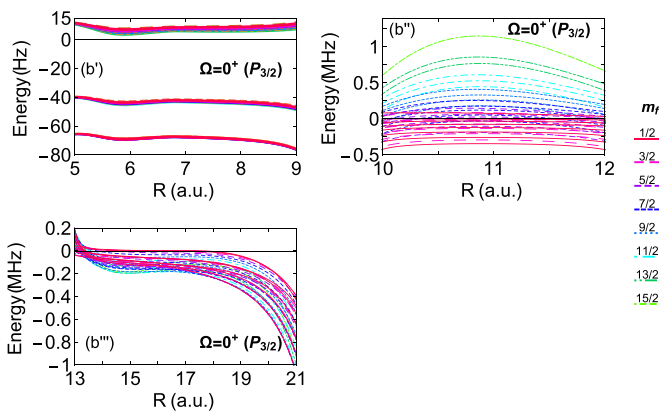
FIG. 11. (Color online) Zooms of the ^{40}\text{KCs} 0^+(P_{3/2}) DPECs of Fig. 8(b) for ranges of R in between the peaks marking the transition from one Hund's case a character to the other.
