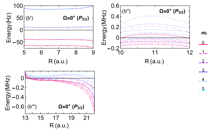
FIG. 9. (Color online) Zooms of the ^{39}\text{KCs} 0^+(P_{3/2}) DPECs of Fig. 7(b) for ranges of R in between the peaks marking the transition from one Hund's case a character to the other.
