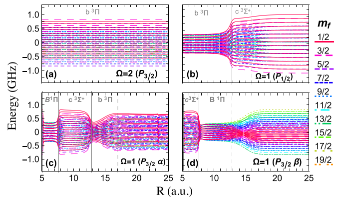
FIG. 6. (Color online) Same as Fig. 5, but for ^{40}\text{KCs} . Each panel contains 72 curves (see Table I).
