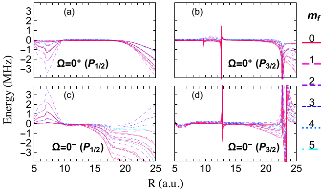
FIG. 7. (Color online) Difference potential-energy curves for \Omega = 0 states in ^{39}\text{KCs} for every value of |m_f| indicated by the color code. Each panel contains 18 curves (see Table I).
