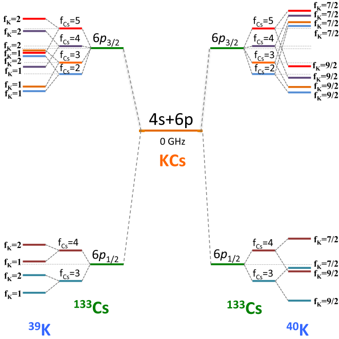
FIG. 3. (Color online) Scheme of the asymptotic molecular hyperfine structure of the bosonic ^{39}\text{KCs} and fermionic ^{40}\text{KCs} molecules at the \text{K}(4^2S_{1/2}) + \text{Cs}(6^2P_{1/2,3/2}) dissociation limit. Energy spacings are not on scale, but the energy-level order is meaningful. Exact energy splittings are reported in the Appendix.
