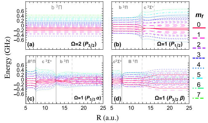
FIG. 5. (Color online) Difference potential-energy curves for \Omega = 2, 1 states in ^{39}\text{KCs} for every value of |m_f| indicated by the color code. Each panel contains 36 curves (see Table I). When appropriate, the dominant Hund's case a state is reported at the top of the panels for each interval between two crossings of Hund's case a potential-energy curves (indicated by solid vertical lines). The dashed lines at large R roughly locate the distance beyond which Hund's case a states are strongly mixed by spin-orbit interaction.
