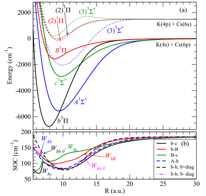
FIG. 1. (Color online) (a) Hund’s case a potential-energy curves of the excited electronic states correlating to the \text{K}(4^2S) + \text{Cs}(6^2P) (solid lines) and \text{K}(4^2P) + \text{Cs}(6^2S) (dashed lines) dissociation limits. The B and c curves cross at R^{Bc} = 7.65 a.u., the b and A curves cross at R^{bA} = 9.55 a.u., and the b and c states cross at R^{bc} = 12.84 a.u. (b) The relevant R -dependent spin-orbit coupling terms associated with the curves dissociating to \text{K}(4^2S) + \text{Cs}(6^2P) (1 a.u. \equiv a_0 = 0.0529177 nm).
