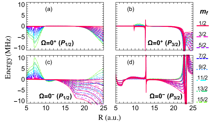
FIG. 8. (Color online) Difference potential-energy curves for \Omega = 0 states in ^{40}\text{KCs} for every value of |m_f| indicated by the color code. Each panel contains 36 curves (see Table II).
