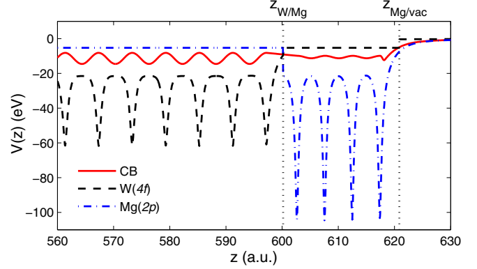
FIG. 2. (Color online) Effective potentials for conduction-band and W( 4f ) and Mg( 2p ) core-level electrons for a 4 ML Mg/W(110) adsorbate-substrate system.
