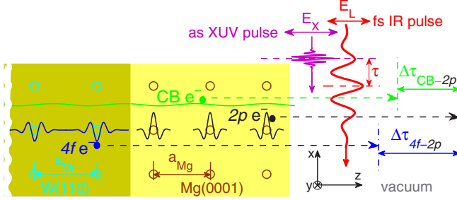
FIG. 1. (Color online) Schematic of attosecond streaking spectroscopy from the Mg/W(110) adsorbate-substrate system.
